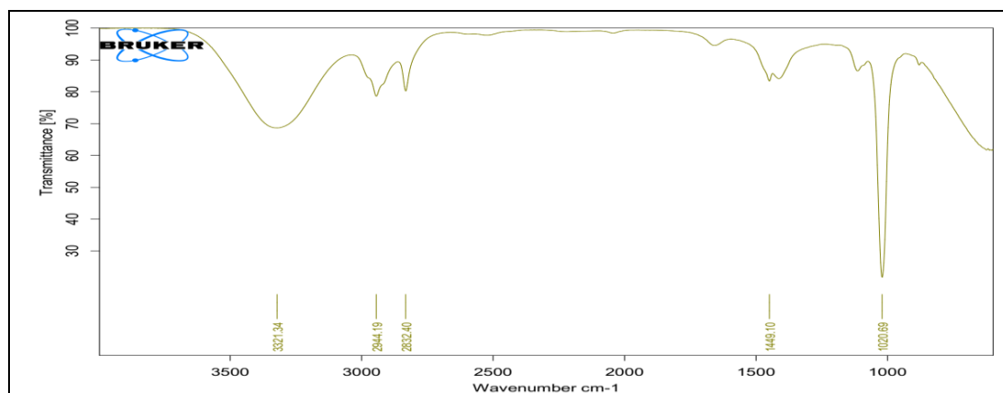
Figure 4.5: FTIR spectra of pure drug.
