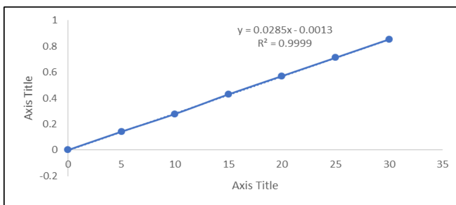
Figure 4.2: Calibration curve of galangin in methanol.
