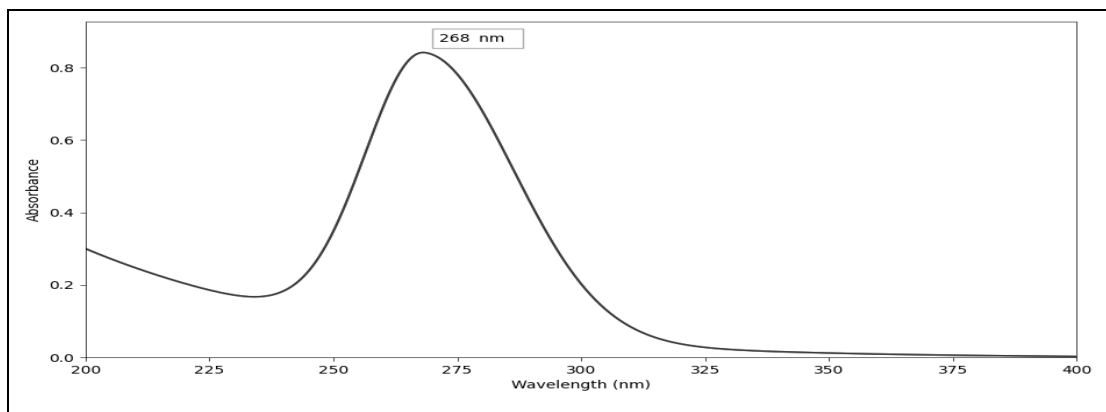
Figure 4.1: Scanning absorbance maxima of galangin (268 nm)
