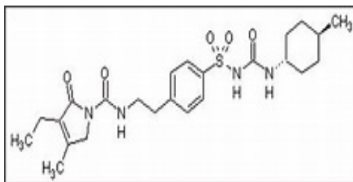
Figure 1: Chemical structure of Glimepiride.
