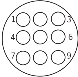
Cabin side connector Type AMP 182645-1 or similar Female (sockets)
