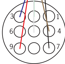
Faucet side connector Type AMP 206705-4 Male (Pins) Include Oras delivery
