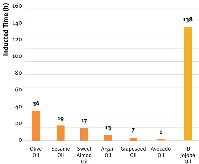
The oxidative stability was determined using Rancimat methods at 110° C in collaboration with Agricultural Research Organization - the Volcani Center, Israel
