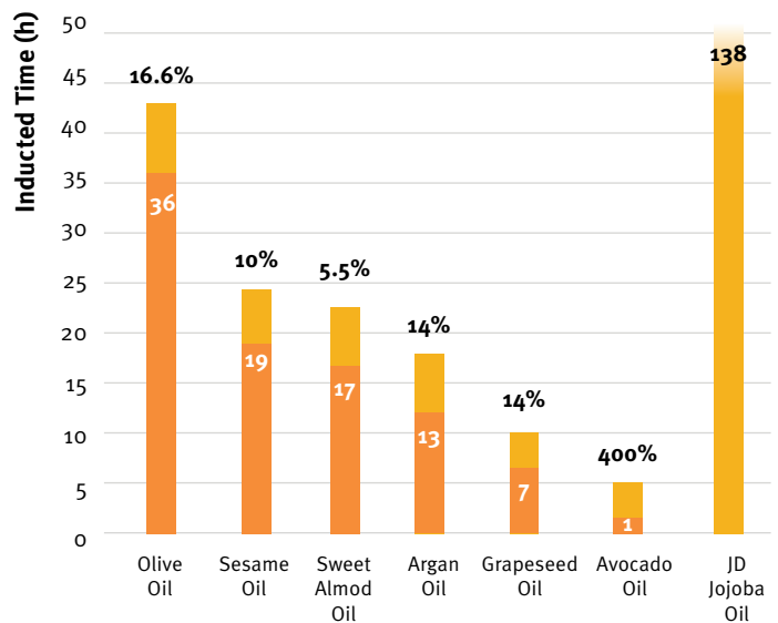
The oxidative stability was determined using Rancimat methods in collaboration with Agricultural Research Organization - the Volcani Center, Israel
