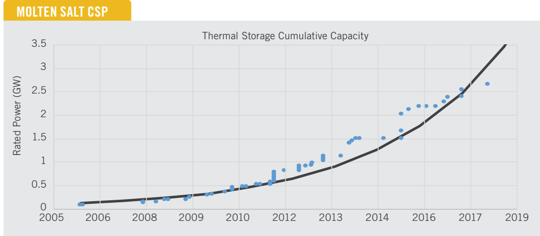
Figure 8: Molten salt CSP compared to a 41 %/year CAGR
