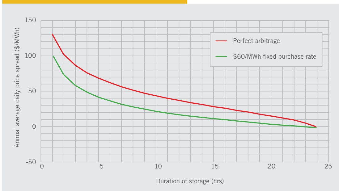
Figure 32: Average price spread for perfect foresight price arbitrage as a function of duration of storage
