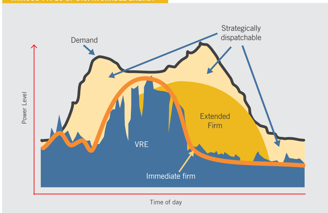
Figure 33: Illustrative use of various types of dispatchable renewable generation in combination with VRE to provide flexible and dispatchable renewable energy-based electricity to meet a daily load
