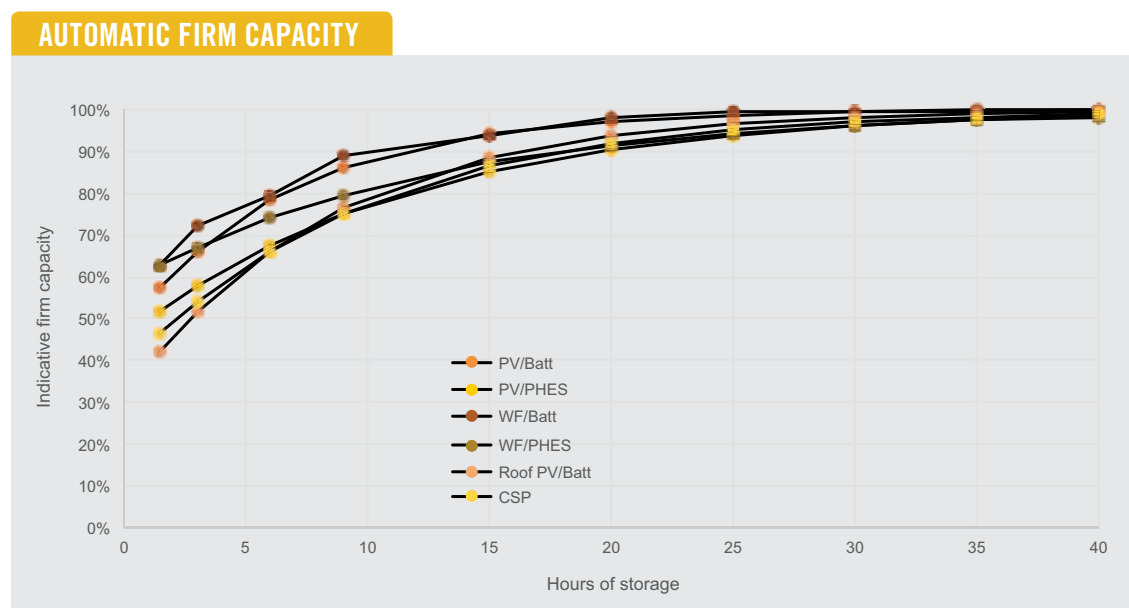
Figure 30: Automatic firm capacity for individual generation and storage options, based on top 10 peak load events in NSW 2016
