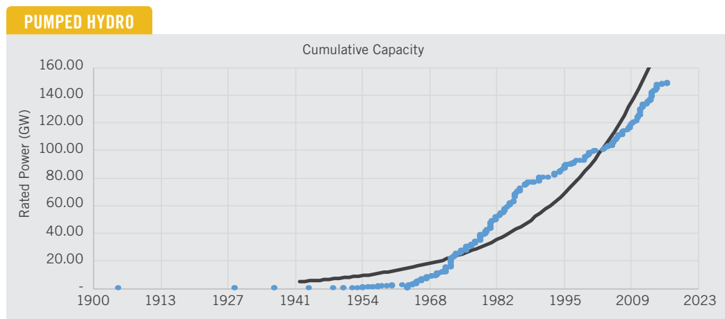
Figure 9: Pumped hydro compared to a 5 %/year CAGR
