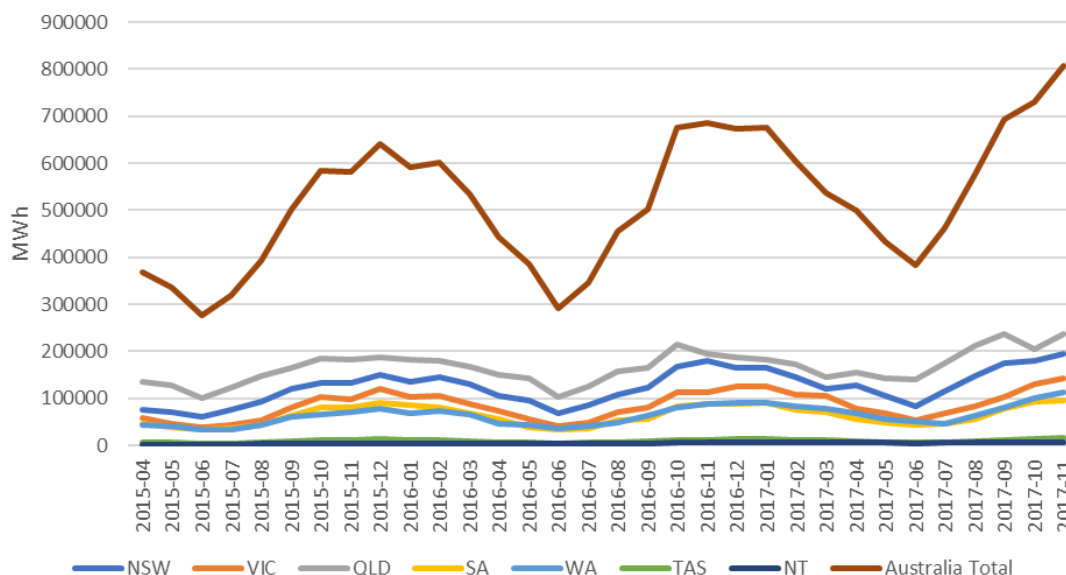
Figure 39: Output from small-scale PV systems in MWh by State 2015-2017, showing seasonal variation and increase over time (Australian PV Institute (APVI) Solar Map, funded by the Australian Renewable Energy Agency, accessed January 2018)
