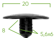
13065 PLASTIC CLIP SETS 15 PCS P/52891
