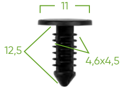
13062 PLASTIC CLIP SETS 20 PCS P/52891
