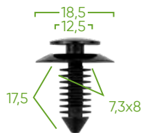
13060 PLASTIC CLIP SETS 5 PCS P/52891
