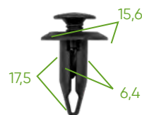
13066 PLASTIC CLIP SETS 5 PCS P/52891
