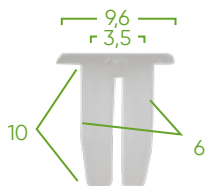
13059 PLASTIC CLIP SETS 20 PCS P/52891
