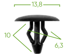
13067 PLASTIC CLIP SETS 25 PCS P/52891
