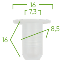
13071 PLASTIC CLIP SETS 10 PCS P/52892
