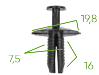
13073 PLASTIC CLIP SETS 5 PCS P/52892
