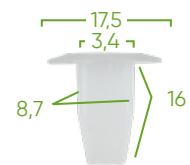
13097 PLASTIC CLIP SETS 3 PCS P/52895
