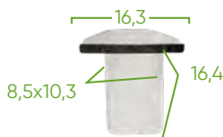
13095 PLASTIC CLIP SETS 6 PCS P/52895
