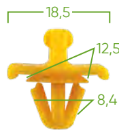
13120 PLASTIC CLIP SETS 60 PCS P/52897
