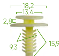
13144 PLASTIC CLIP SETS 25 PCS P/52900
