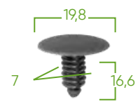
14412 PLASTIC CLIP SET 10PCS FOR 53715
