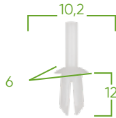
14455 PLASTIC CLIP SET 12PCS FOR 53718
