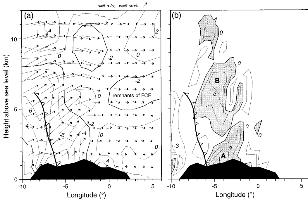
Fig. 7. Vertical/zonal section of (a) the mean slope of isentropes, (\partial z/\partial x)_\theta , and the average wind vector within this plane, and (b) the quantity (I_{Fx}/|I_{Fx}|)[\partial I_{Fx}/\partial t]_{rel} , along the 41^\circ – 42^\circ latitude band (Fig. 3) for 8 August 1992, 0600 UTC, according to the ECMWF analysis. The orography of Iberia, smoothed as in the ECMWF-model, is also shown. In (a) isopleths of (\partial z/\partial x)_\theta are indicated by solid lines, labeled in units of 10^{-3} . In (b) isopleths of (I_{Fx}/|I_{Fx}|)[\partial I_{Fx}/\partial t]_{rel} are labeled in units of 10^{-7} \text{ s}^{-1} . The letters A and B indicate separate areas of intense frontogenesis (see the text for further discussion).
