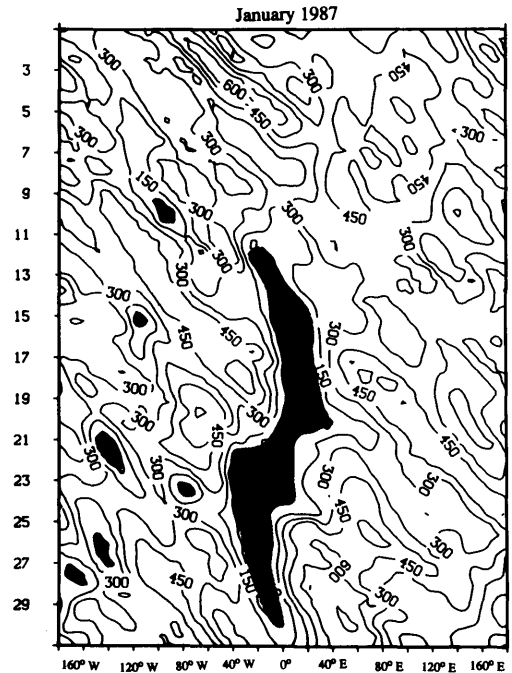
Fig. 1. Hovmöller diagram displaying the Lejenäs-Økland Index for January 1987. See text for definition. The abscissa is longitude (degrees) and the ordinate is time (days). The contour interval for the LO index values is 150 gpm. The shaded regions are values less than zero.
