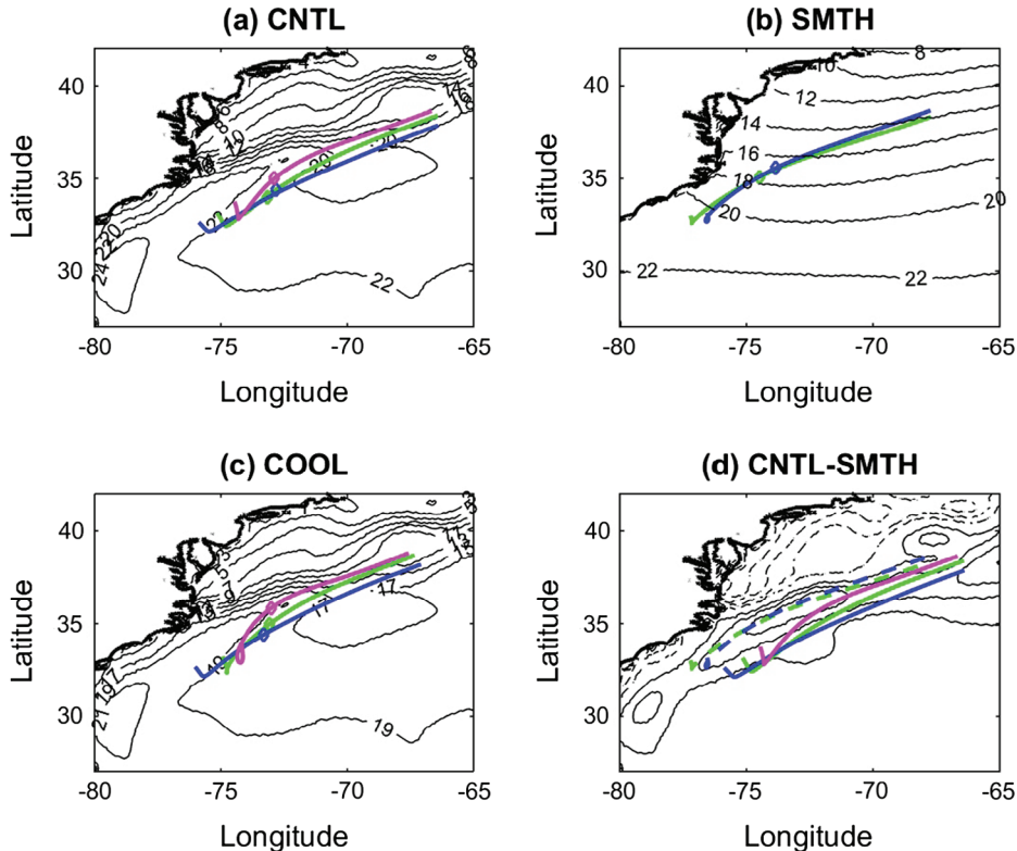
Fig. 1. SST (contoured every 2^\circ\text{C} ) used in experiment (a) CNTL (b) SMTH and (c) COOL. Panel (d) gives the difference CNTL-SMTH (contoured every 1.5^\circ\text{C} , positive continuous, negative dashed). The colour curves in panels (a), (b) and (c) are the average horizontal trajectories for the respective experiments, as discussed in Section 2.2 (magenta: z_0 \geq 7 km, green: 5 \text{ km} \leq z_0 < 7 km, blue: z_0 < 5 km). The diamonds on these curves indicate the average locations when parcels leave the boundary layer. The colour curves in (d) indicate the CNTL (continuous lines) and SMTH (dashed lines) mean trajectories, reproduced from panel (a) and (b), respectively.
