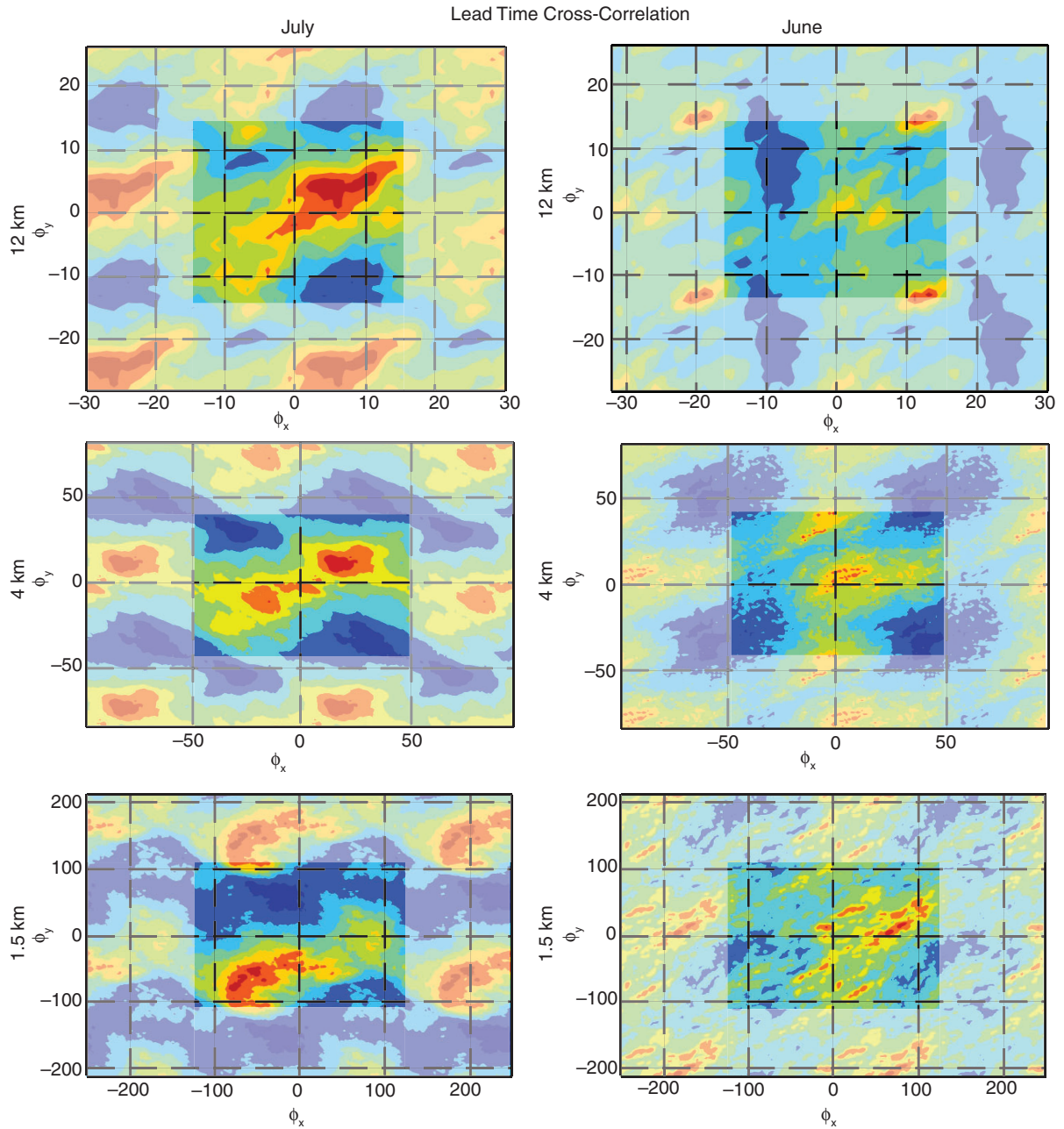
Fig. 6. Cross-correlation between the precipitation fields from the 12-hour lead time and the 36-hour lead time for the 12 km (top), 4 km (middle) and 1.5 km (bottom) runs for July 2007 (left) and June 2007 (right). Red indicates a high correlation, blue shows a low correlation. The axes are the number of grid boxes shifted in each direction. The artificial periodicity is shown in the masked area.
