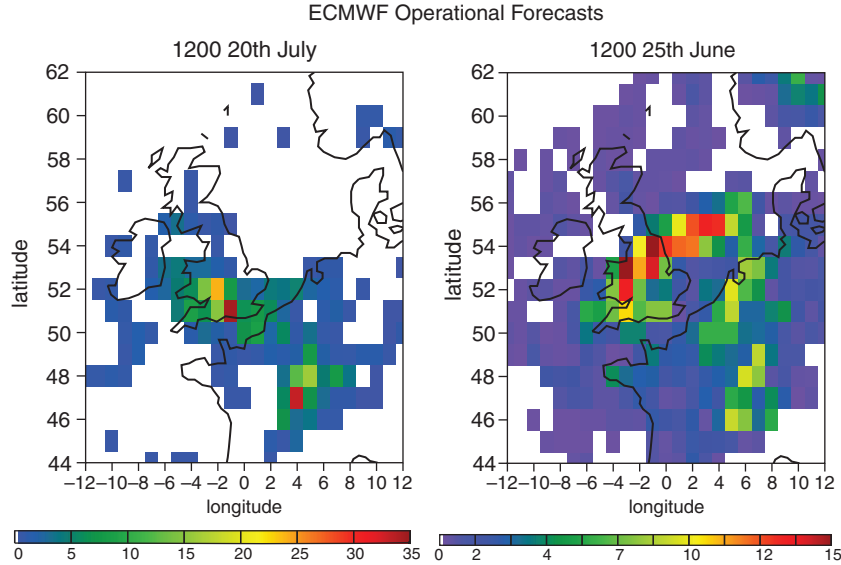
Fig. 7. Six-hour precipitation accumulation for 1200 on the 20th July 2007 (left) and for 1200 on the 25th June 2007 (right) from the ECMWF Operational Forecast, the Operational Analysis was used to drive the LAM. Units are mm, the minimum accumulation shown is 0.5 mm.
