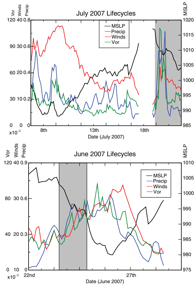
Fig. 3. Lifecycles of the July (top) and June (bottom) 2007 events, including the precursor event. The black line represents Mean Sea Level Pressure (MSLP, hPa), the blue line precipitation (precip, mm/hr), the red line winds (m/s) and the green line 850 hPa relative vorticity (vor, \times 10^{-5}/s ), taken from the ECMWF Operational Analysis. The grey area is when the storm was over the UK.
