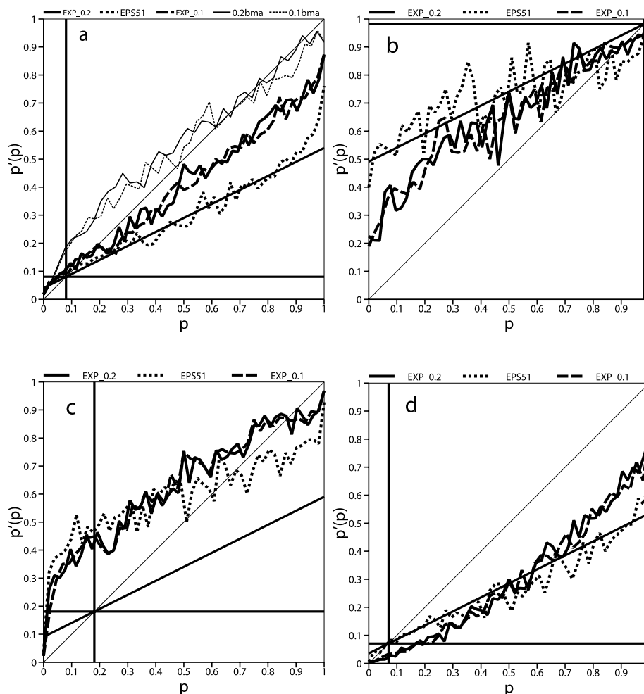
Fig. 4. Reliability diagrams, i.e. the conditional frequency p' of observed events with predicted probabilities p . Thick lines: 52 member GLAMEPS (EXP0.2, continuous); 51 member operational EPS (dotted), 44 member GLAMEPS (EXP_0.1, dashed). Events: +42 h predicted wind speed > 10 \text{ ms}^{-1} (a); +42 h predicted 2 m temperature > -10 \text{ }^\circ\text{C} (b); > 10 \text{ }^\circ\text{C} (c); and +18 to +24 h predicted 6-hourly accumulated precipitation > 1 \text{ mm} (d). Thin lines in (a): BMA calibrated wind speeds EXP_0.2 (continuous) and EXP_0.1 (dashed). The diagonal is perfect reliability; the half diagonal is zero brier skill score (no skill), horizontal and vertical lines is the observed frequency over the period (no resolution).
