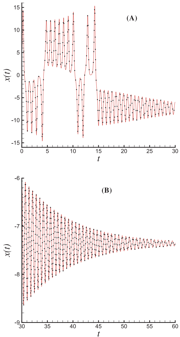
Fig. 11. (a) Comparison of x(t) in case of \sigma = 10, R = 21.5, b = -8/3 with the initial state x = y = z = 5 by means of \tau = 0.01 LTU and the M th-order scheme (3) based on truncated Taylor series in the interval 0 \leq t \leq 30 . Line: M = 30 ; Symbols: M = 40 . (b) The same, but in the interval 30 \leq t \leq 60 .
