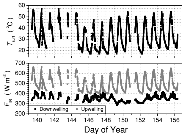
Fig. 1. Time-series of the surface temperature (upper panel) and of the upwelling (lower panel; grey) and downwelling (black) broad-band thermal radiation, measured by pyrometers at Ouarzazate airport. Day of year 139 corresponds to 19 May; 152 is 1 June; 156 is 5 June, 2006.
