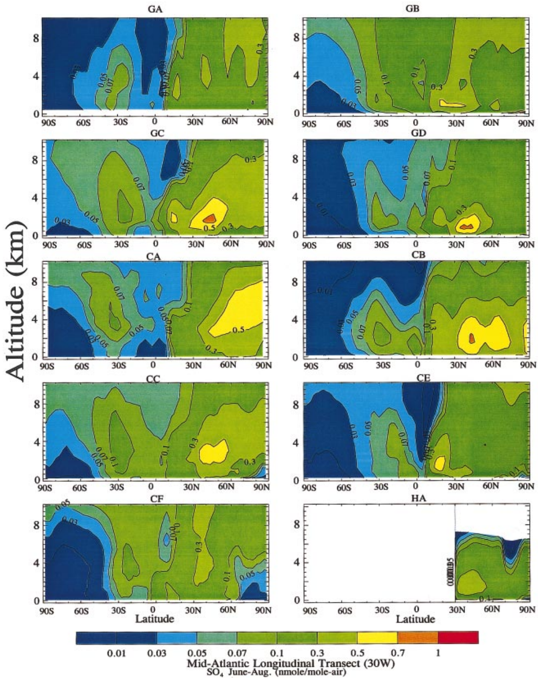
Fig. 9. A longitudinal profile comparison of model simulated mean SO 4 - mixing ratio (nmole/mole-air) along a mid-Atlantic transect (30°W) for the northern hemispheric summer (June–August).
