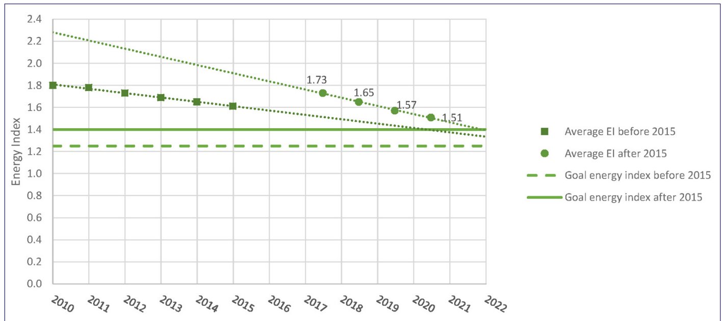
Figure 3: Progress of the average energy index (EI NV) in the Dutch non-profit housing sector.
