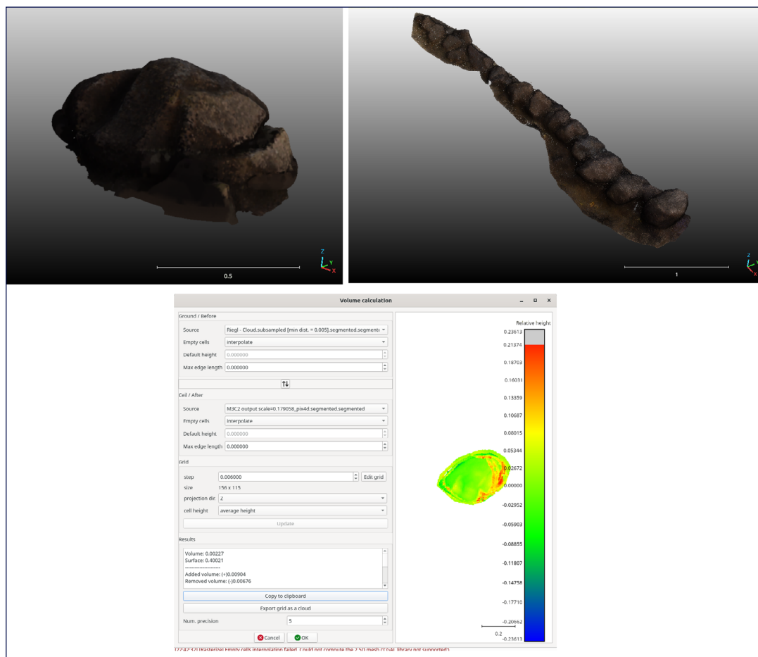
Figure 8 From left to right: The Riegl point cloud of a rock used in the comparisons; the Riegl point cloud of the stone row used in the comparisons and a view of the Calculate 2.5D Volume tool.
