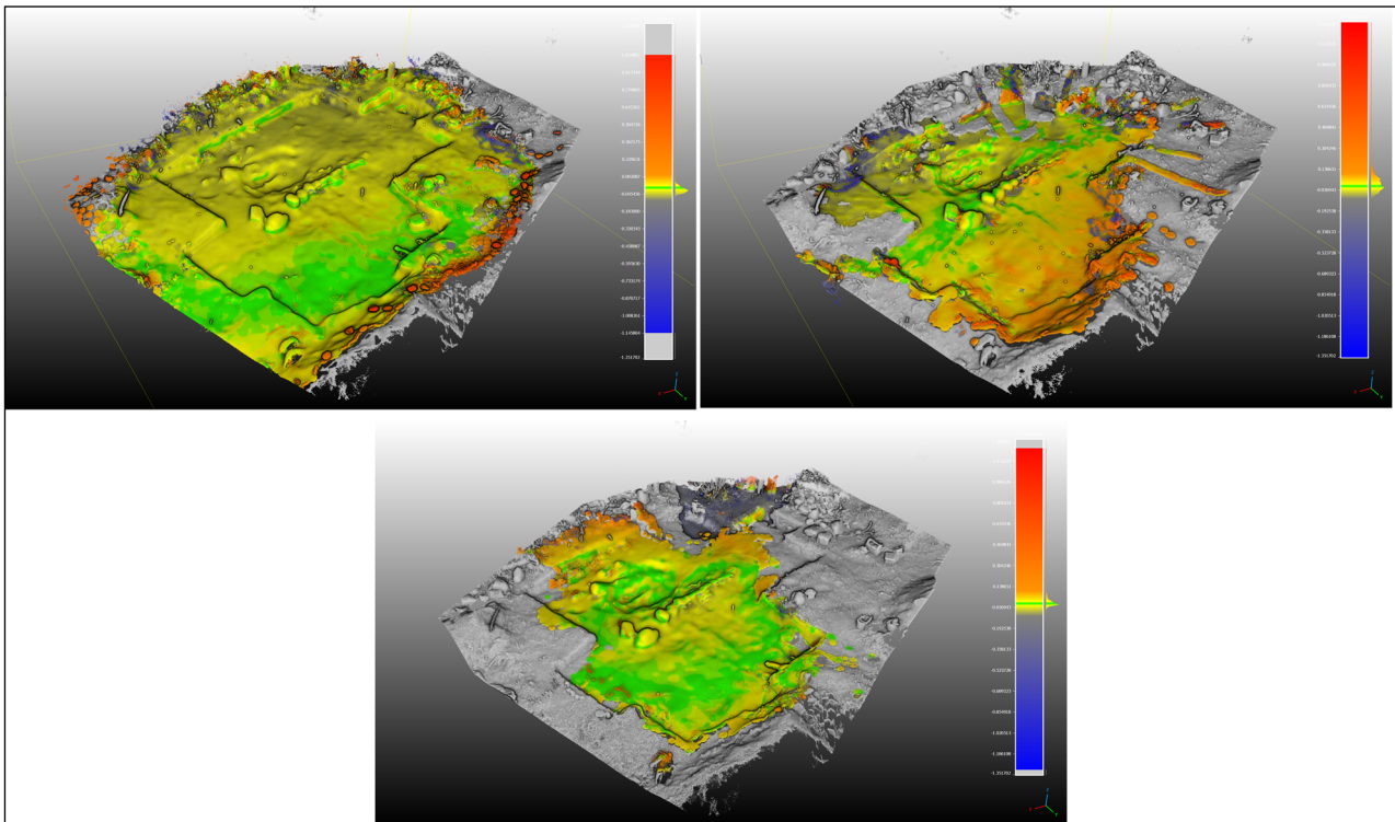
Figure 7 Point clouds colored using Scalar field values of M3C2 comparison. In descending order: DJI Osmo and RealityCapture, iPhone and Pix4D and iPhone and Scaniverse.
