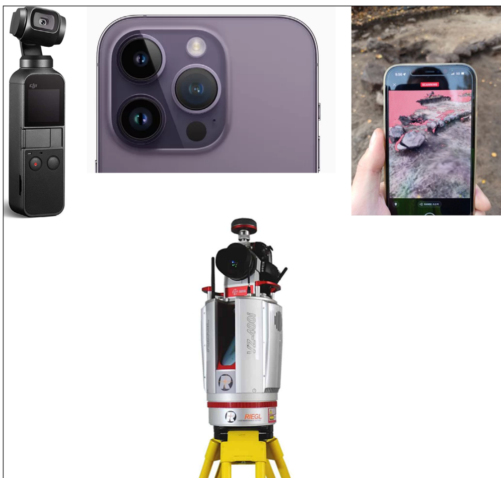
Figure 2 From left to right: DJI Osmo, iPhone LiDAR sensor location, iPhone scanning with onscreen visual feedback, and VZ-400i terrestrial laser scanner.
