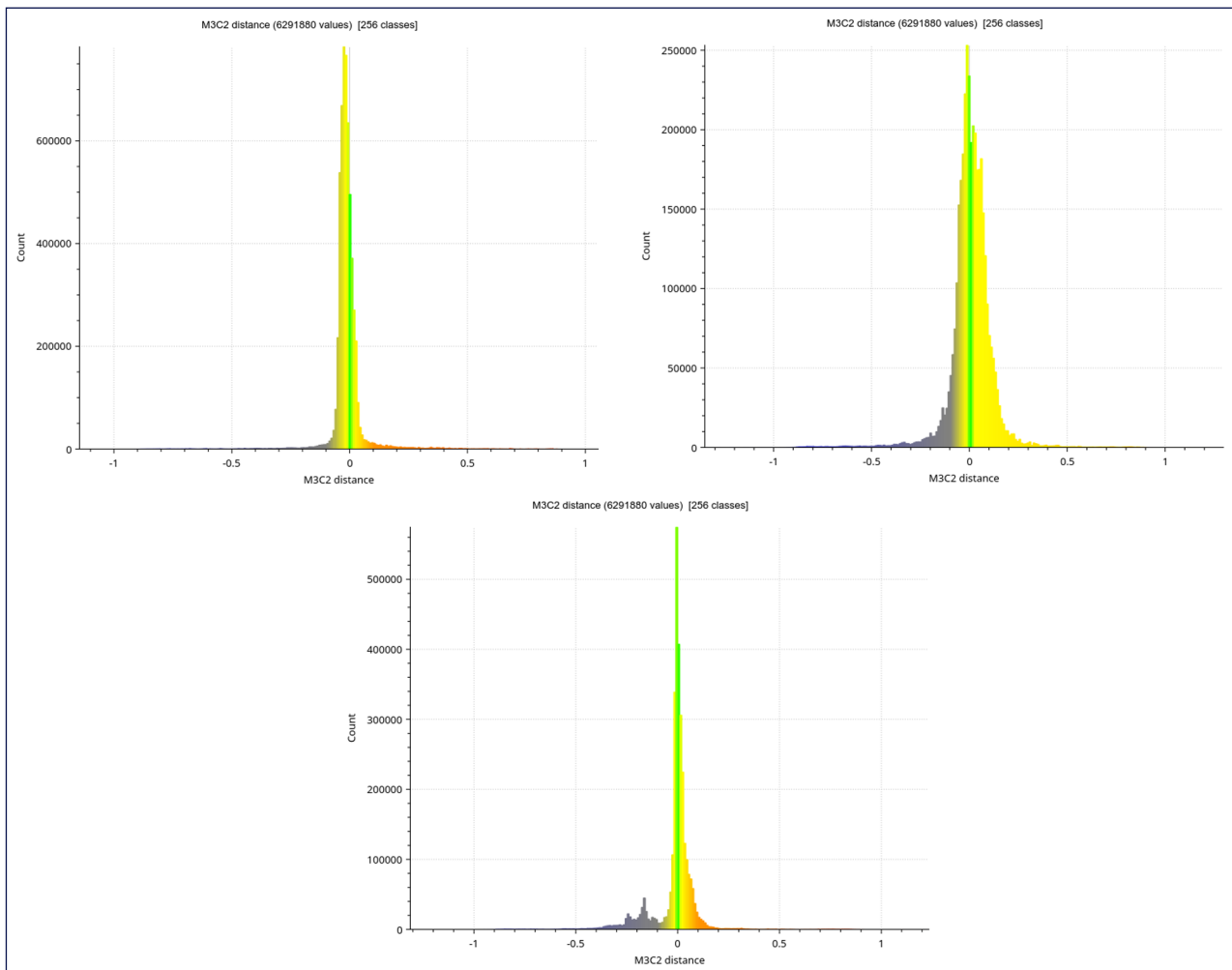
Figure 6 Histograms in descending order: DJI Osmo and RealityCapture, iPhone 12 Pro and Pix4D and iPhone 12 Pro and Scaniverse. M3C2 distance indicates the difference to the reference cloud in meters, whereas Count indicates the number of points falling into that M3C2 range.
