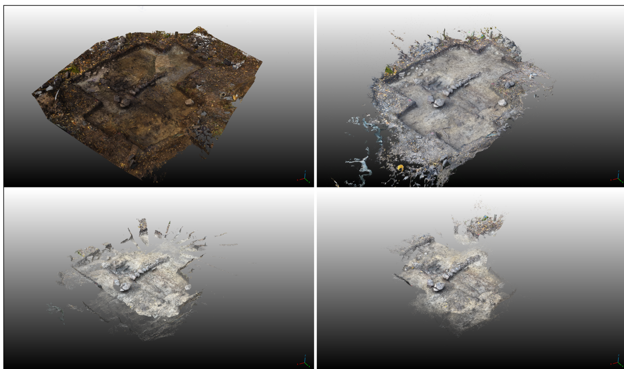
Figure 5 Textured views of four clouds. From left to right: Riegl VZ-400i (cropped), DJI Osmo + RealityCapture, iPhone 12 Pro + Pix4D and iPhone 12 Pro + Scaniverse.
