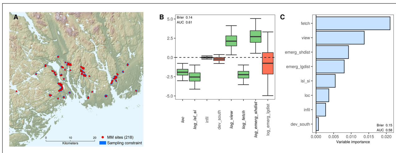
Figure 8: Middle Mesolithic – Buffer sample. A) Map overview. B) Logistic regression, percentile bootstrap. C) Random forest, permutation variable importance.
