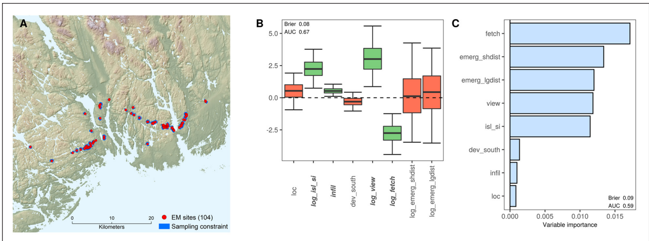
Figure 6: Early Mesolithic – Buffer sample. A) Map overview. B) Logistic regression, percentile bootstrap. C) Random forest, permutation variable importance.
