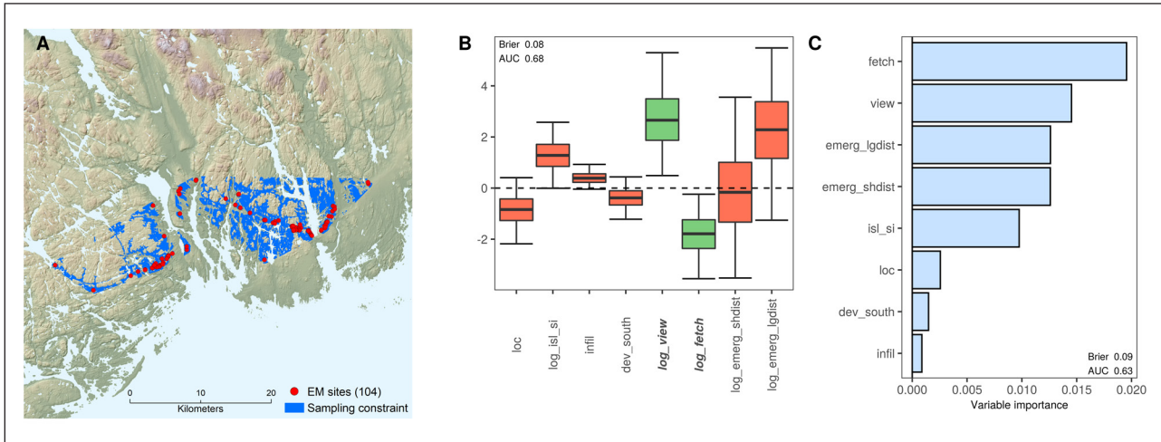
Figure 5: Early Mesolithic – Hull sample. A) Map overview. B) Logistic regression, percentile bootstrap. C) Random forest, permutation variable importance.
