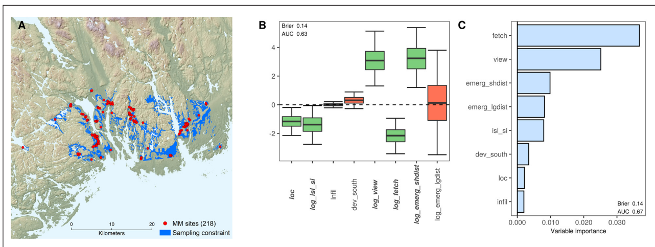
Figure 7: Middle Mesolithic – Hull sample. A) Map overview. B) Logistic regression, percentile bootstrap. C) Random forest, permutation variable importance.
