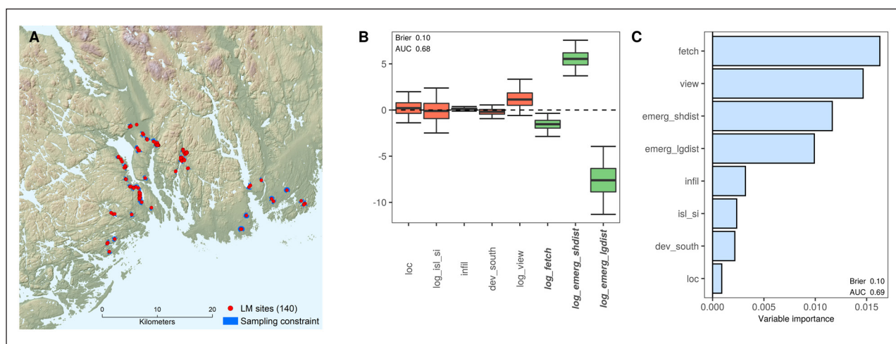
Figure 10: Late Mesolithic – Buffer sample. A) Map overview. B) Logistic regression, percentile bootstrap. C) Random forest, permutation variable importance.
