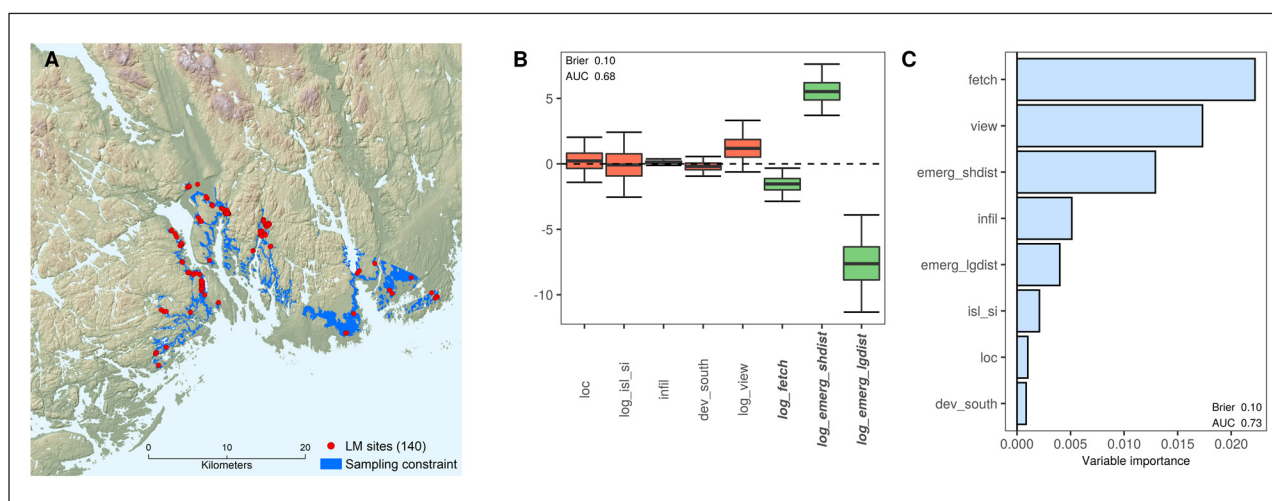
Figure 9: Late Mesolithic – Hull sample. A) Map overview. B) Logistic regression, percentile bootstrap. C) Random forest, permutation variable importance.
