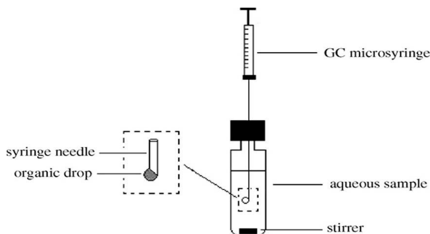
Fig 2. Direct-immersion single-drop microextraction
