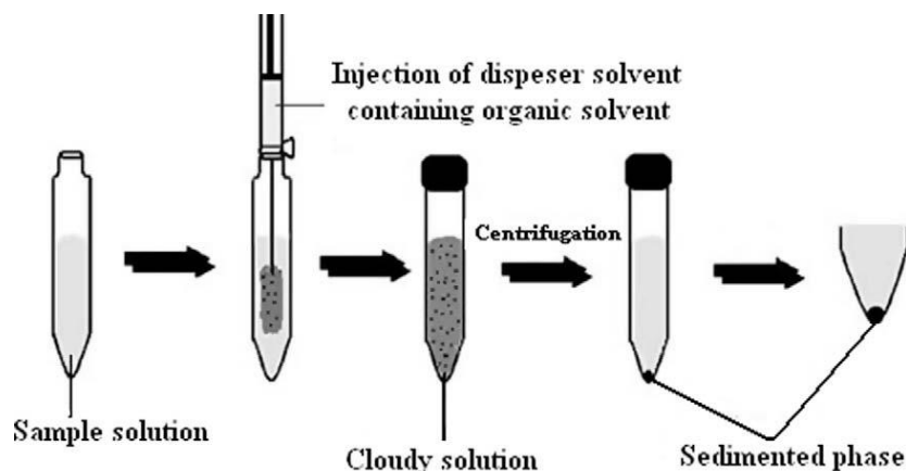
Fig 3. Different steps in dispersive liquid-liquid microextraction
