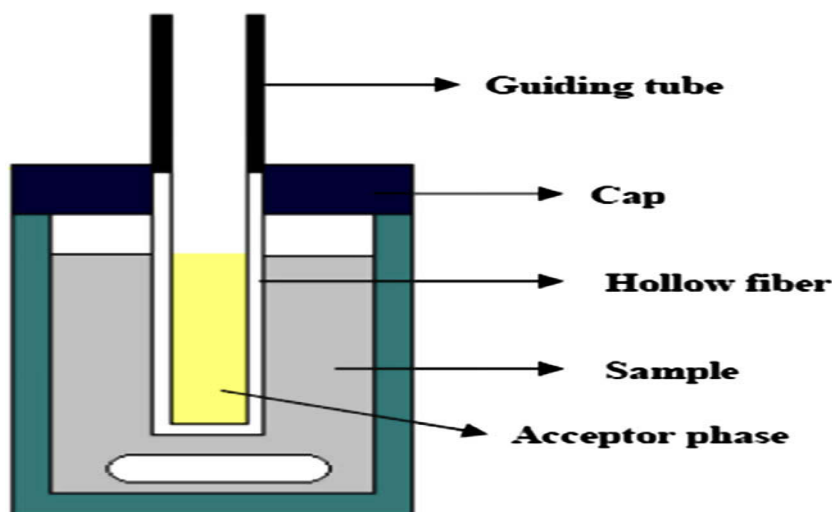
Fig 4. Principle of hollow-fiber liquid phase microextraction
