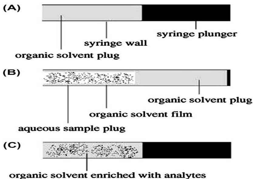
Fig 1. Operation of dynamic liquid-phase microextraction
