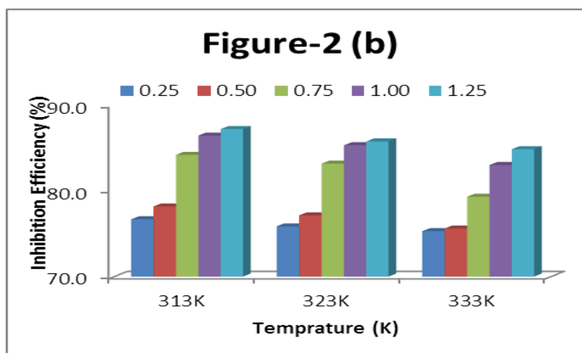
Figure 2(b): Effect of inhibition concentration of Jasud leaf extract for mild steel in 1M HCl at different temperatures for 3h.
