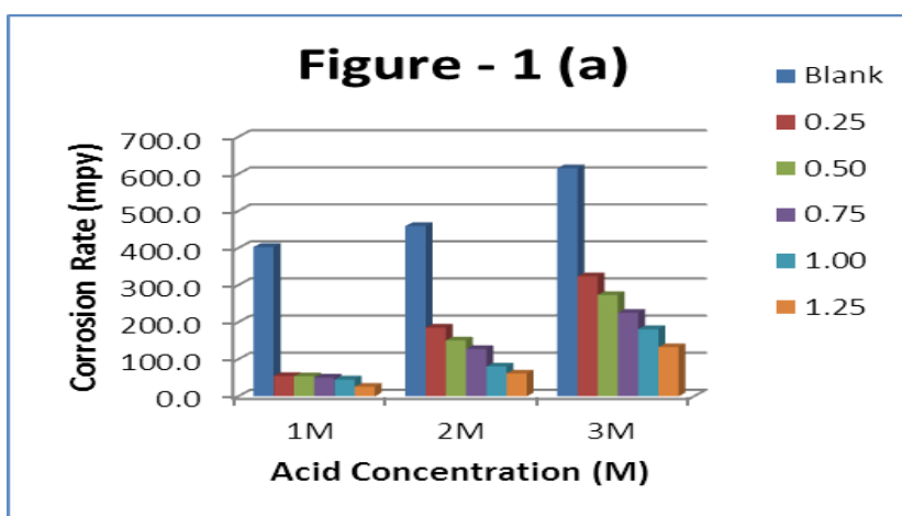
Figure:1(a) Corrosion rate of Jasud leaf extract for mild steel at different acid and inhibitor concentrations for 24 h at 301 K.
