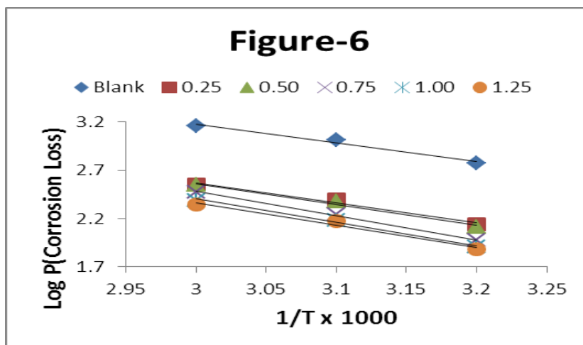
Figure 6: Arrhenius plots for corrosion of mild steel in 1 M HCl in absence and presence of Jasud leaf extract.
