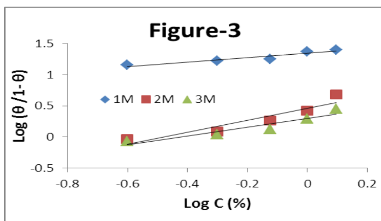
Figure 3: Plot of \log(\theta / (1-\theta)) versus \log C for Jasud leaf extract at different concentrations of HCl for 24 h at 301 K.
