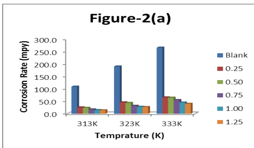
Figure 2 (a): Corrosion rate of Jasud leaf extract for mild steel in 1M HCl at different temperatures for 3h.
