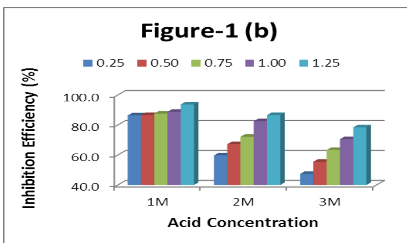
Figure:1(b) Effect of inhibition efficiency of Jasud leaf extract for mild steel at different acid and inhibitor concentrations for 24 h at 301 K.
