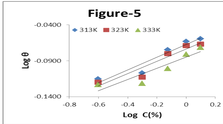
Figure 5: Plot of Log \theta versus Log C for Jasud leaf extract at different concentrations of HCl for 3 h .
