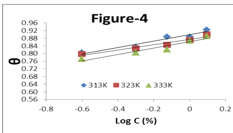
Figure 4: Plot of \theta versus \log C for Jasud leaf extract at different concentrations of HCl for 3h.
