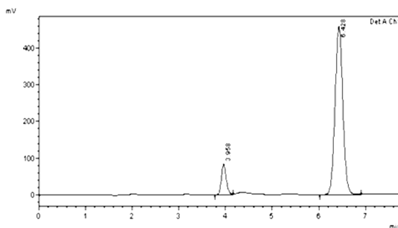
Figure 1. HPLC chromatogram for simultaneous analysis of Clavulanic acid (10 \mu\text{g/ml} ) and Amoxicillin (50 \mu\text{g/ml} )
