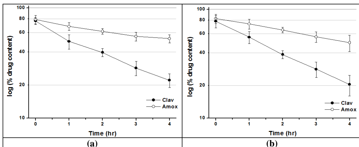
Figure 4. Degradation profiles of Clavulanic acid and Amoxicillin from reconstituted co-amoxiclav injection that stored at 30°C in (a) dark and (b) indoor room light for 4 hours
