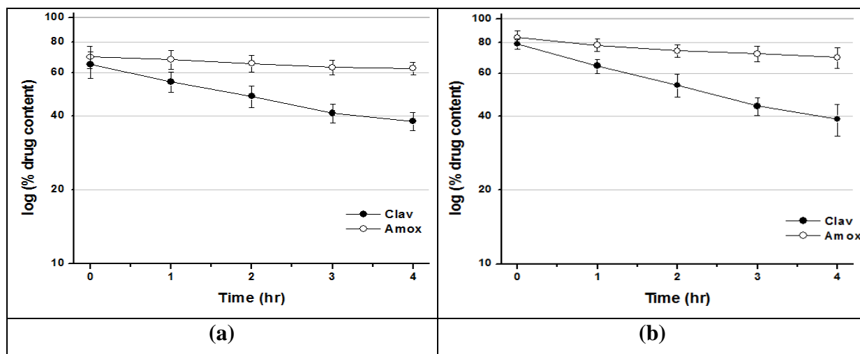
Figure 3. Degradation profiles of Clavulanic acid and Amoxicillin from reconstituted co-amoxiclav injection that stored at 4-8°C in (a) dark and (b) indoor room light for 4 hours
