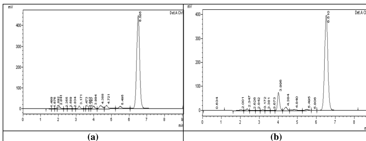
Figure 2. Chromatograms for Co-amoxiclav solutions that subjected to (a) HCl hydrolysis for 2 hrs and (b) thermal degradation for 1 hr on a water bath.
