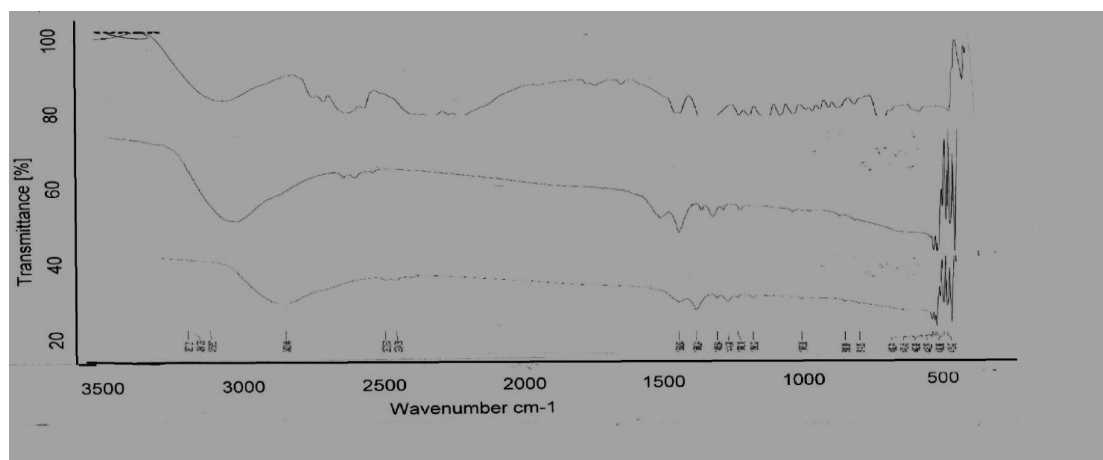
Figure 1: FTIR Spectra of a) Imipramine b) Hibiscus rosa-sinensis c) Imipramine + Hibiscus rosa-sinensis
