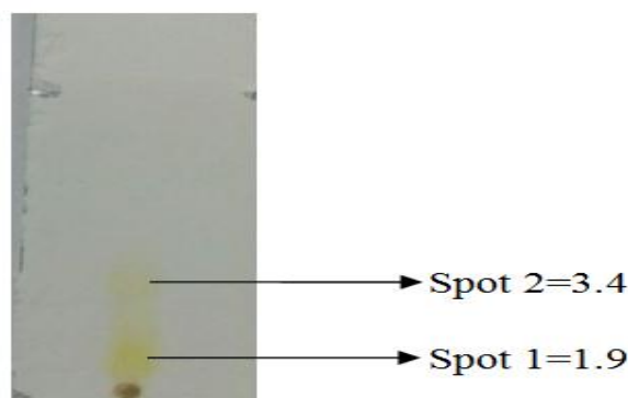
Figure 2: TLC of Aqueous extract of Haridra
