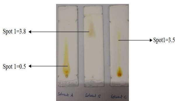
Figure 3: TLC of Hydroalcoholic extract of Haridra .
