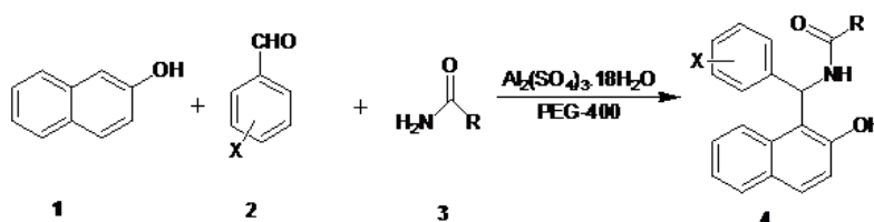
Scheme-1: Synthesis of 1-amidoalkyl-2-naphthols.
