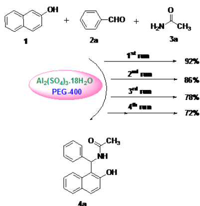
Scheme-2: Recycle study of the catalytic system.
