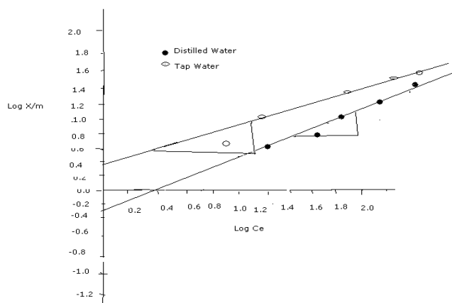
Fig.6: Freundlich Adsorption Isotherm for the Adsorption of Cr (VI); Time: 10Hrs: pH: 1
