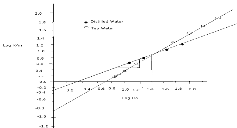
Fig.7: Freundlich Adsorption Isotherm for the Adsorption of Cr (VI); Time: 10Hrs; pH: 2
