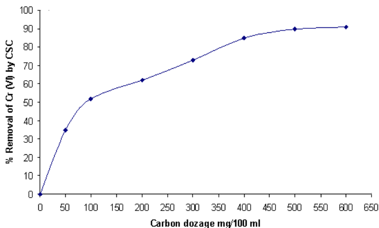
Fig: 3 Effect of Carbon Dosage pH; 1
