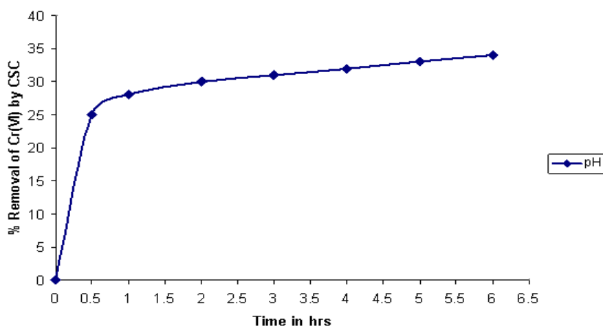
Fig.1: Effect of Time for the Removal of Cr (VI) of Concentration 10mg/L- Carbon Dose 100mg/100mL; pH: 5.0 Effect of pH
