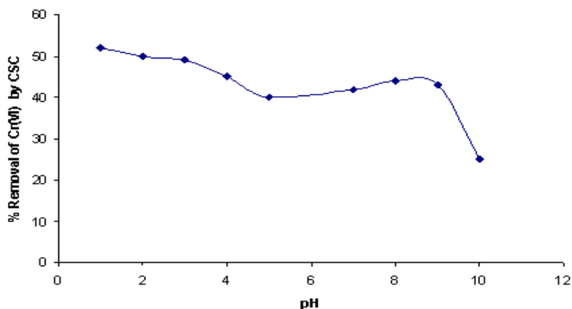
Fig.2: Effect of pH on Adsorption of Cr (VI) of Concentration 10mg /L-Time: 3hrs: Carbon Dose 100mg/100mL; pH: 5.0-9.0
