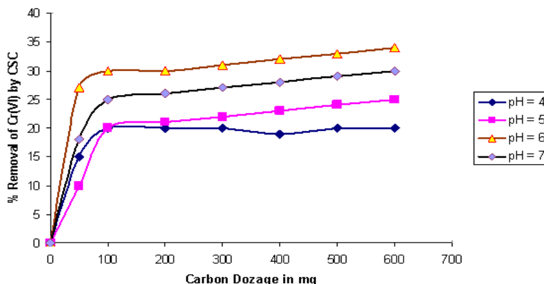
Fig: 5 Effect of Carbon Dosage on Adsorption of Cr (VI) Of Concentration 10mg/L- Time 3Hrs; pH: 4 to 7
