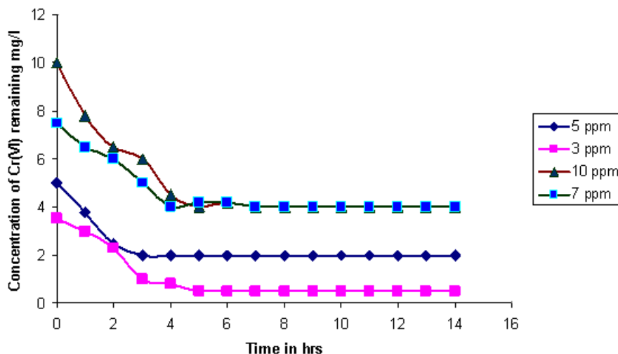
First Order Kinetic Fit for the Adsorption of Cr (V) on CSC
