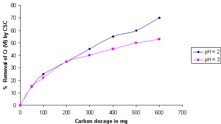
Fig: 4 Effect of Carbon Dosage pH; 2 & 3
