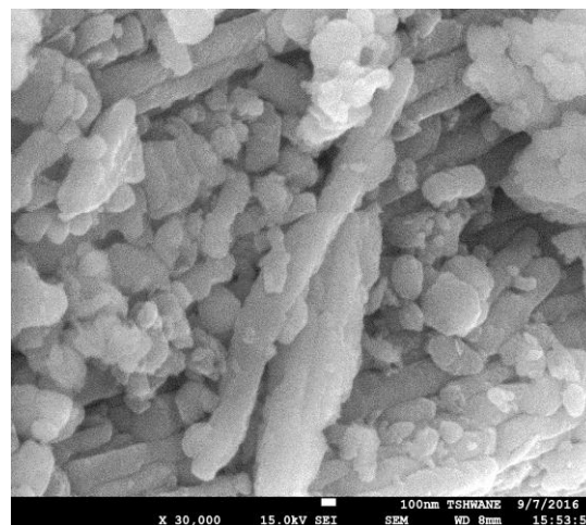
Figure 1: SEM micrograph of chitosan-acacia gum arabic nanoparticles
