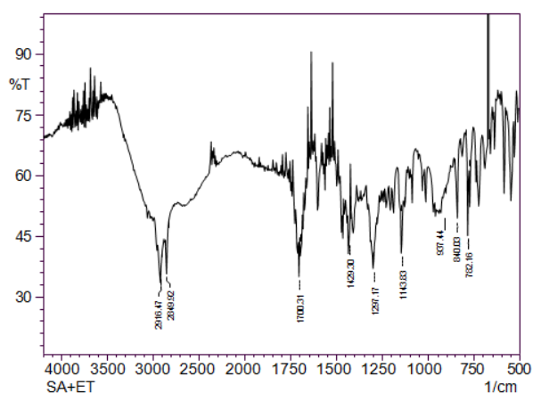
Fig. 7: IR spectrum of Stearic acid + Drug.
