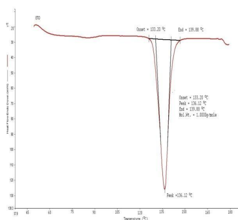
Fig. 9: DSC graph of Enflucixib.
