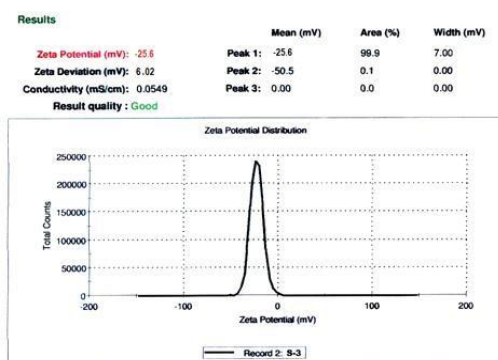
Fig. 3: Zeta potential of SLN-F3 Dispersion.
