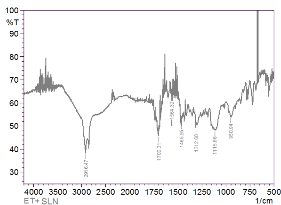
Fig. 8: IR spectrum of Drug loaded SLN.
