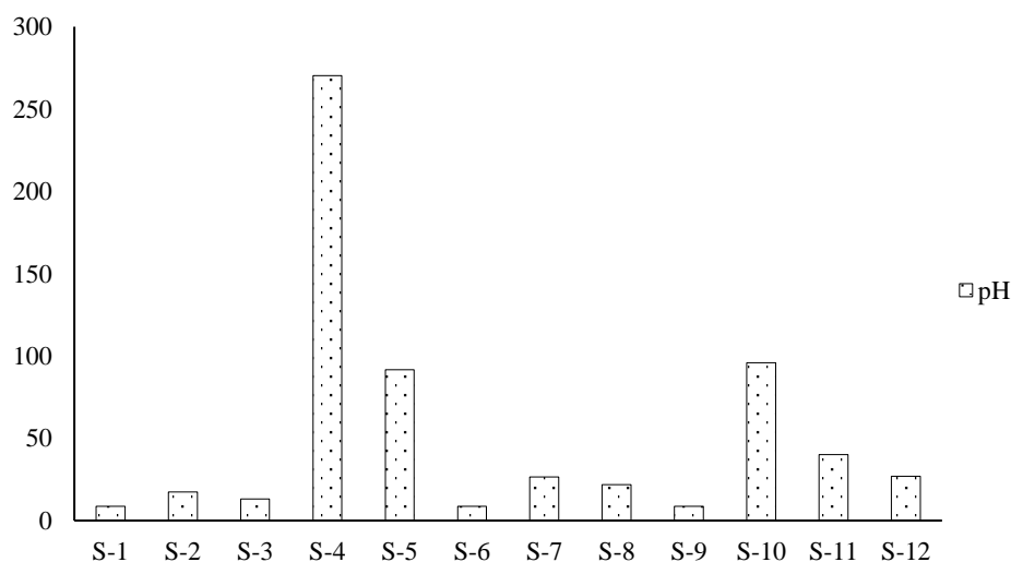
Figure 2. pH.
