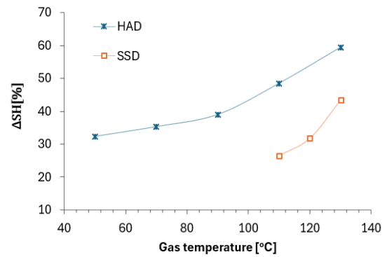
Fig. 13. Shrinkage of dried pear
