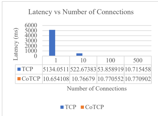
Fig. 11. Latency vs. Number of Connections
