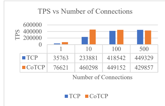
Fig. 8. TPS vs. Number of Connections
