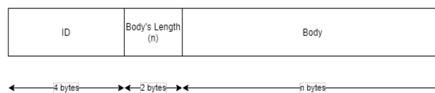
Fig. 4. Message's structure.
