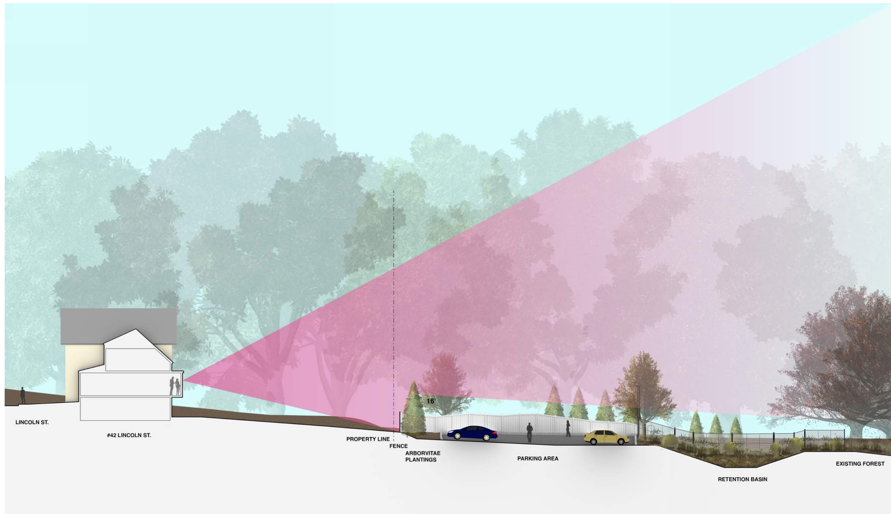
SITE SECTION THROUGH PARKING AREA ARBOR VITAE AT 16 FEET (5 YEARS)
