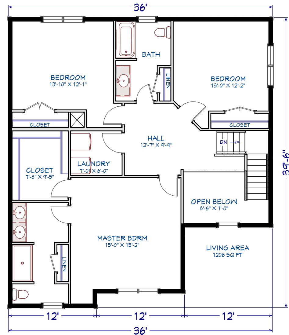
2nd Floor
