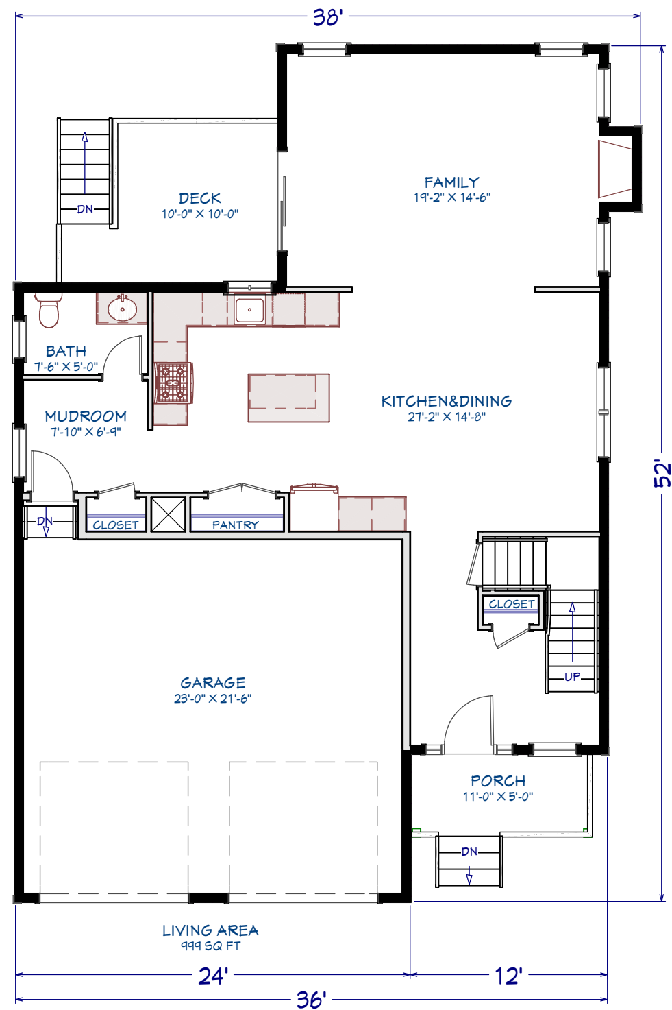
1st Floor
