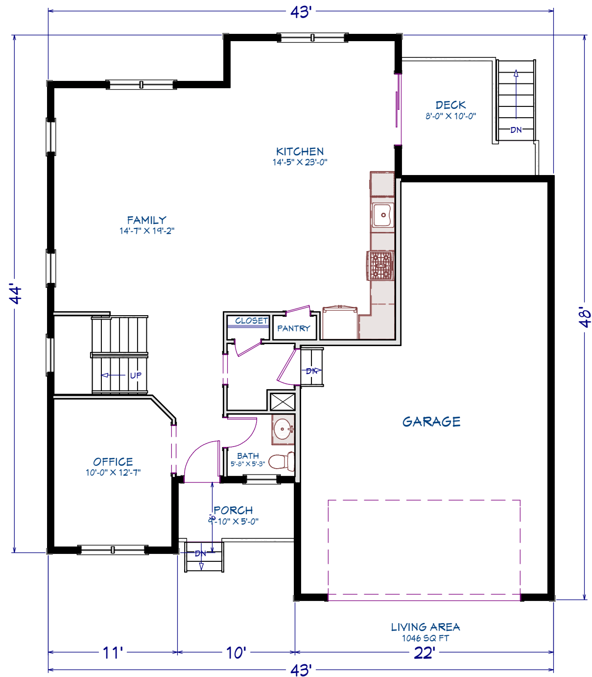
1st Floor
