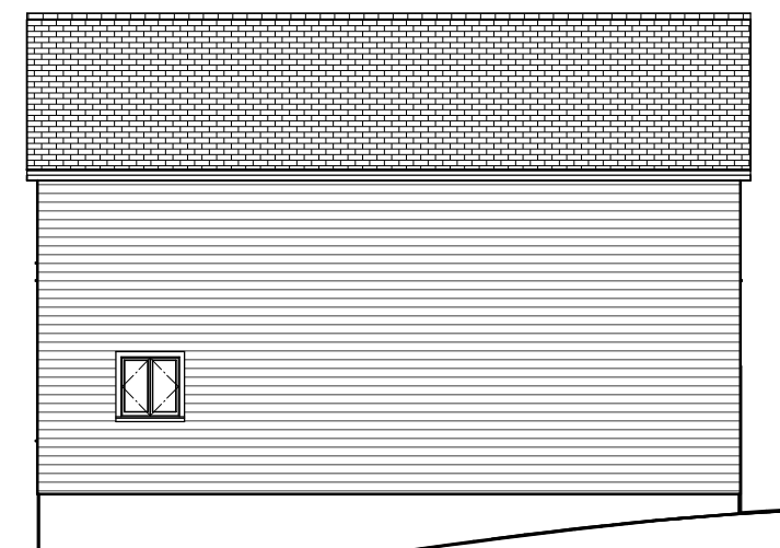
Side Elevation
