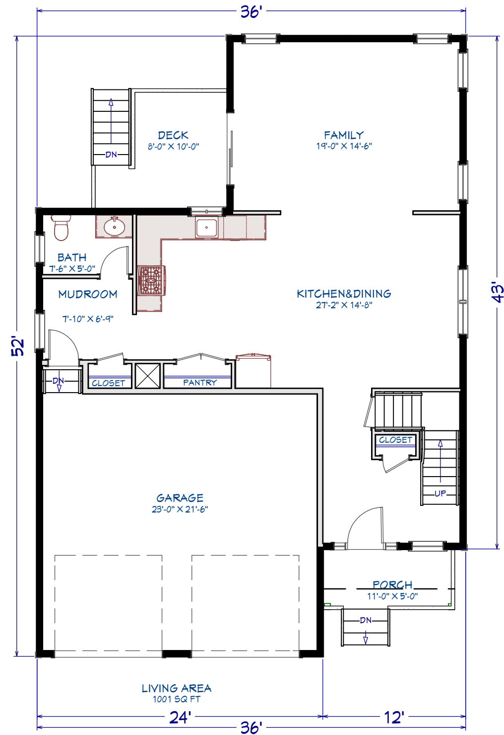
1st Floor
