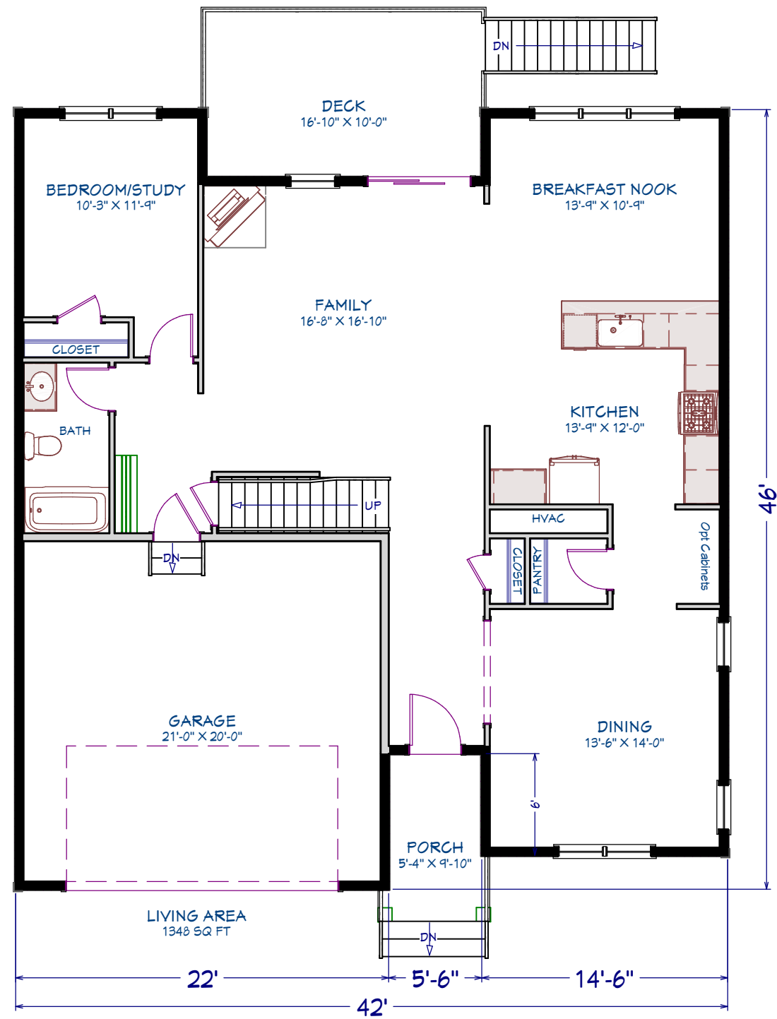
1st Floor
