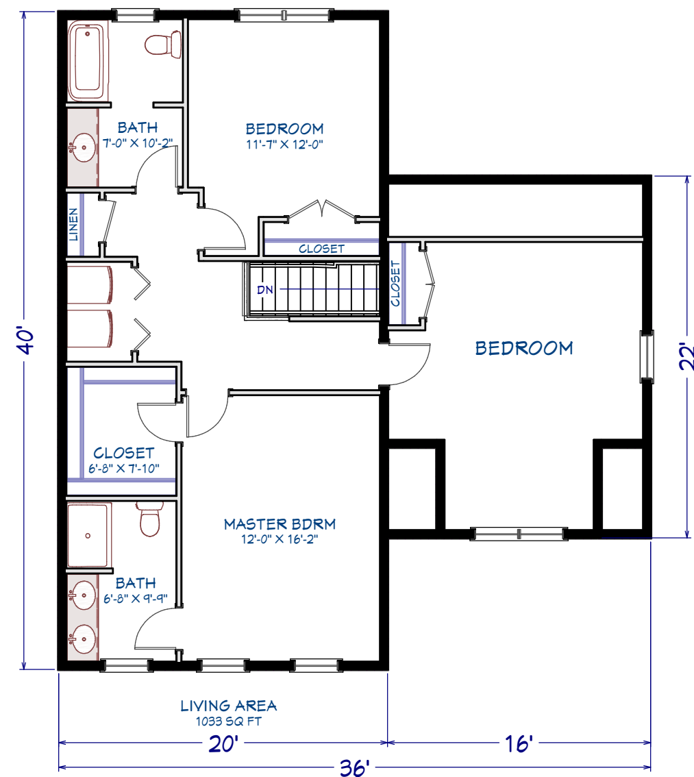
2nd Floor
