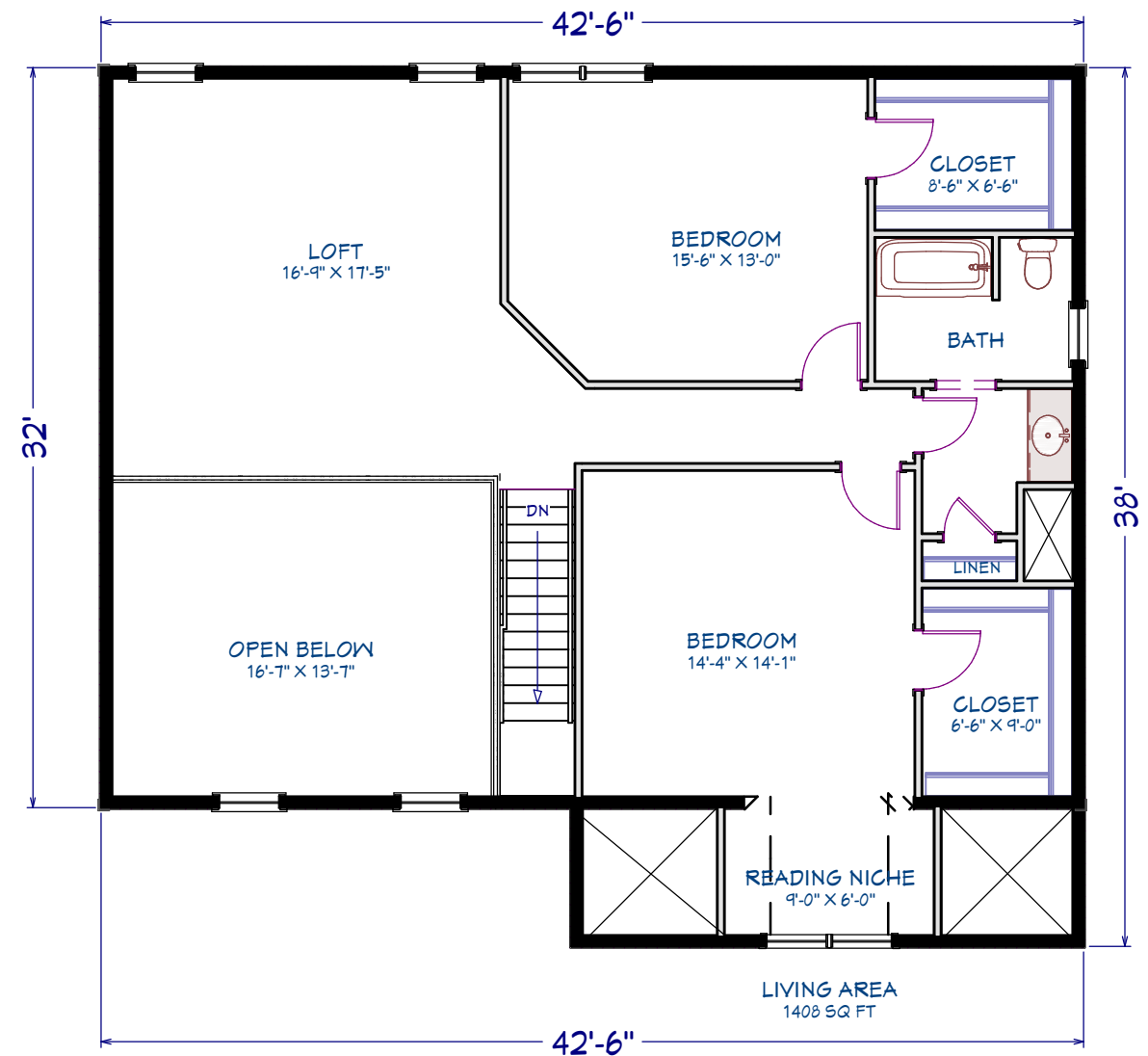
2nd Floor
