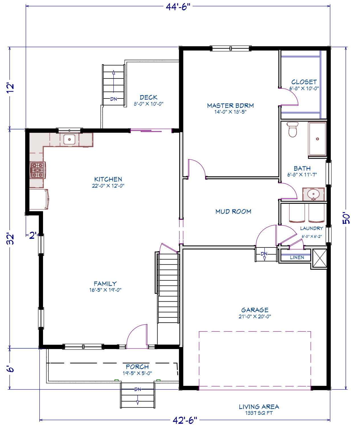
1st Floor
