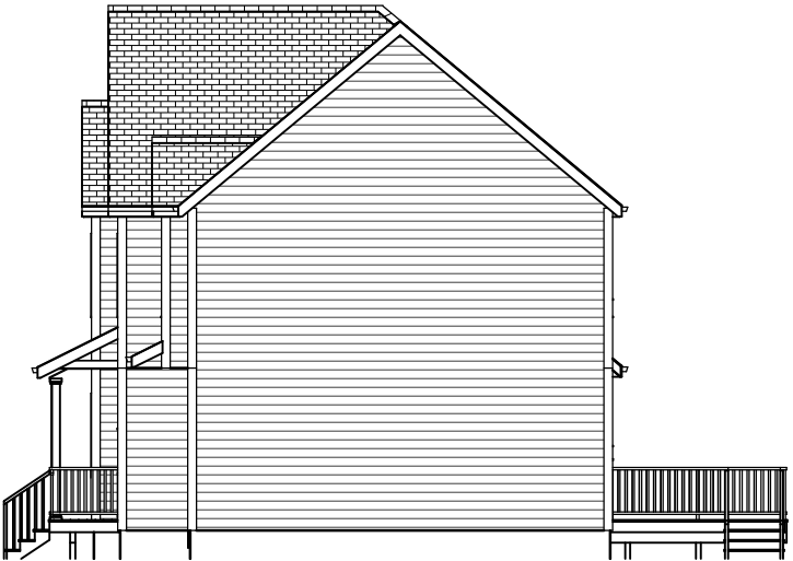
Side Elevation
