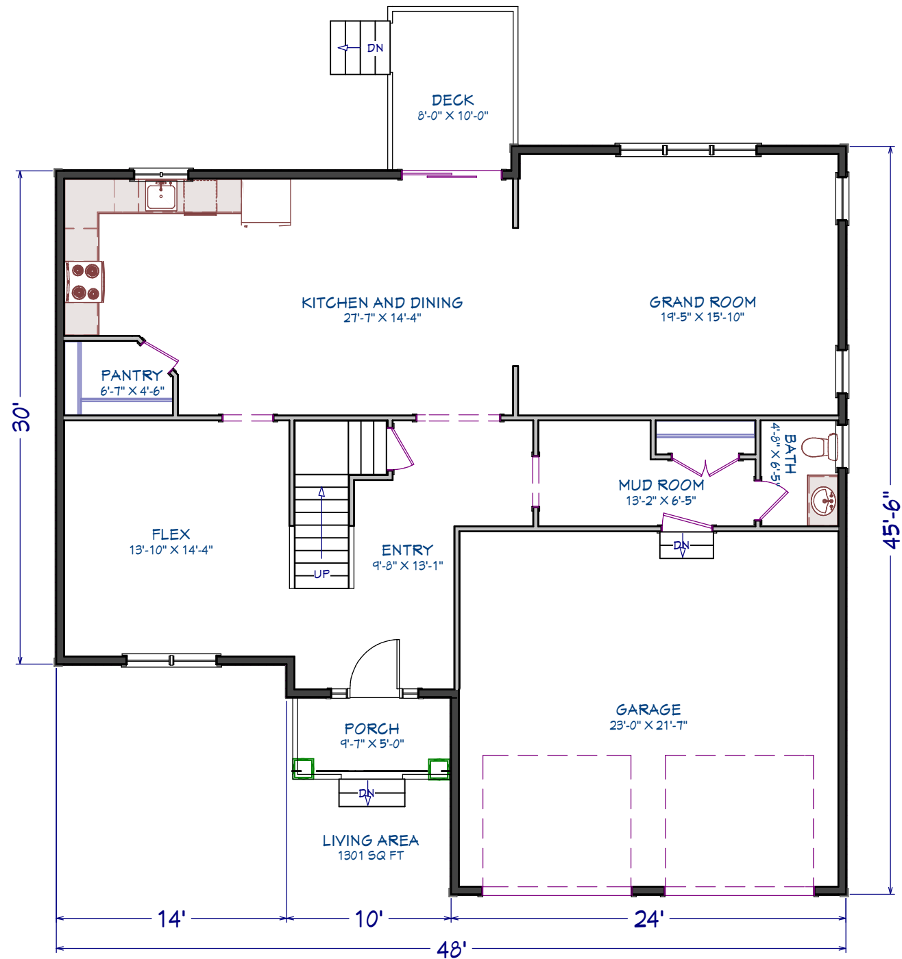
1st Floor
