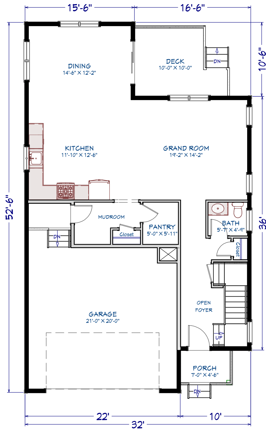
1st Floor
