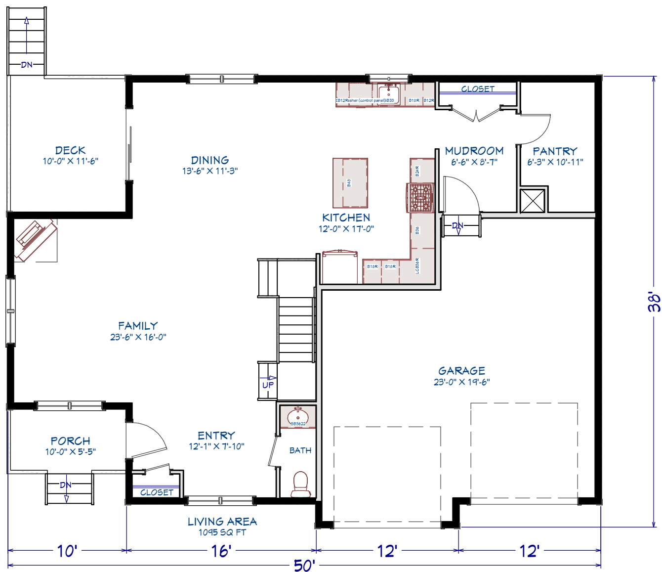
1st Floor
