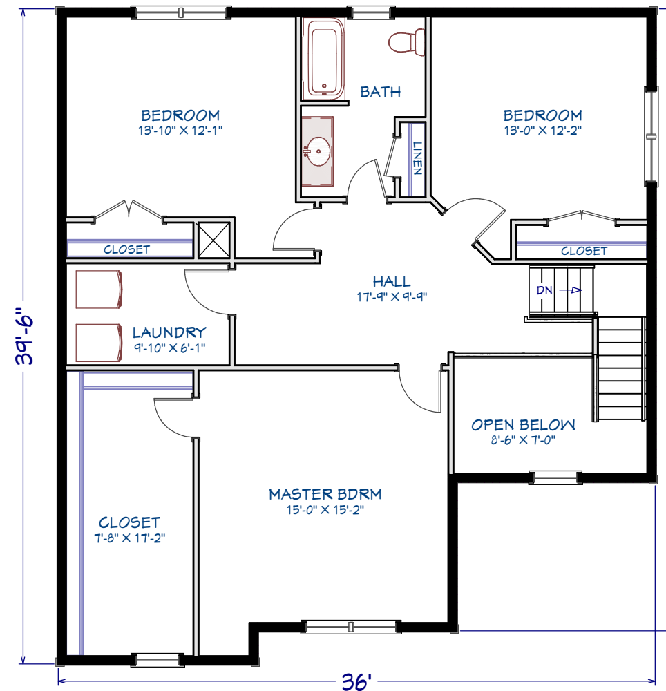
2nd Floor
