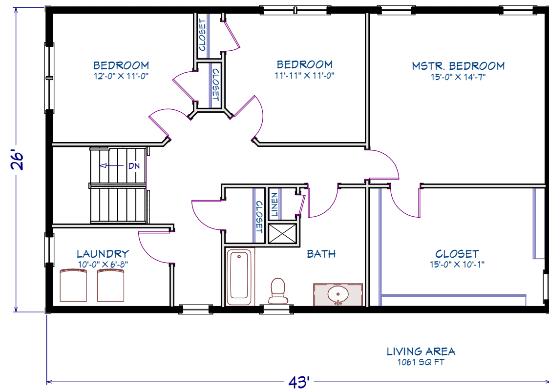
2nd Floor
