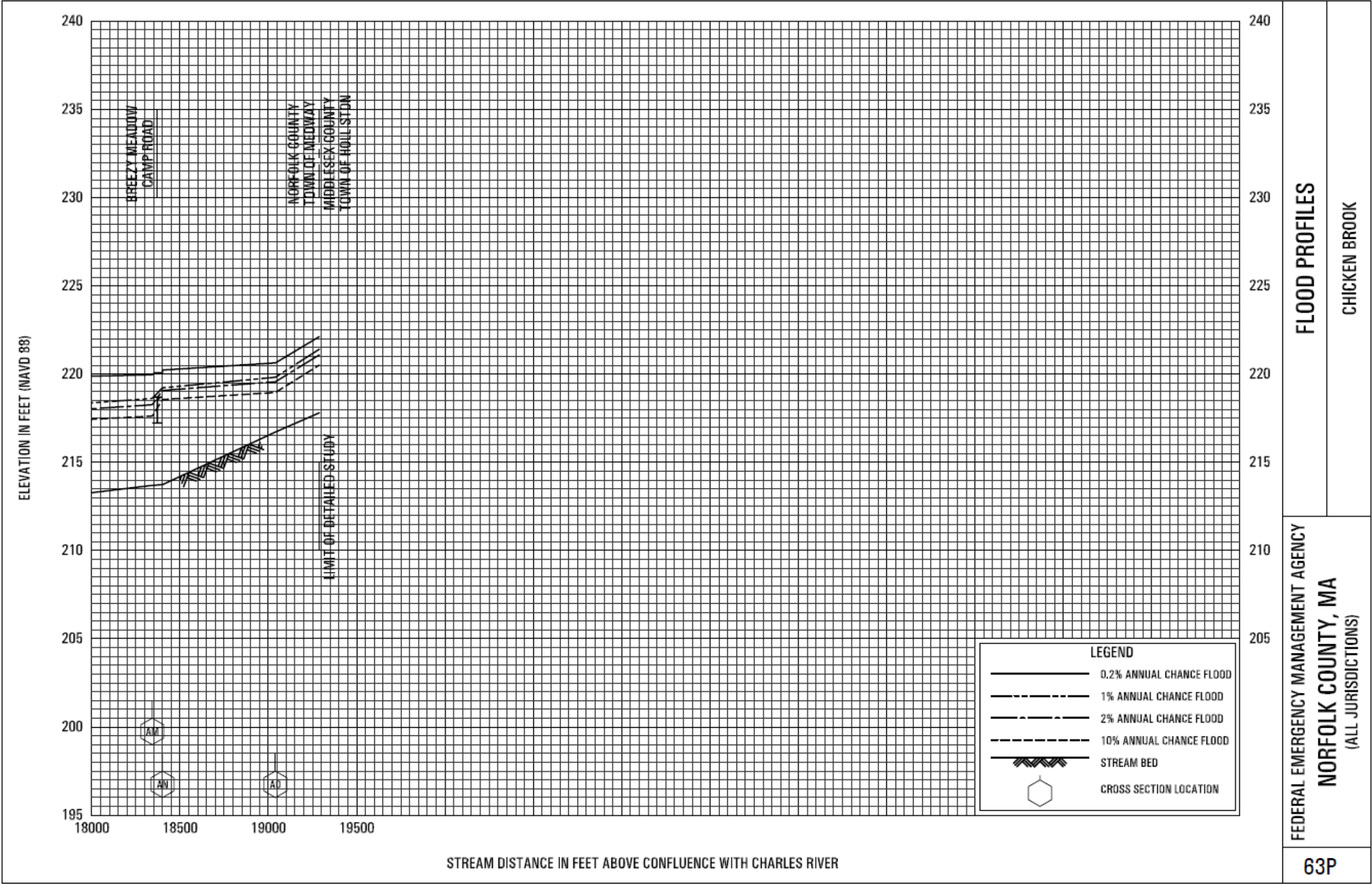
FIS Flood Profile for Chicken Brook in Medway, 63P
