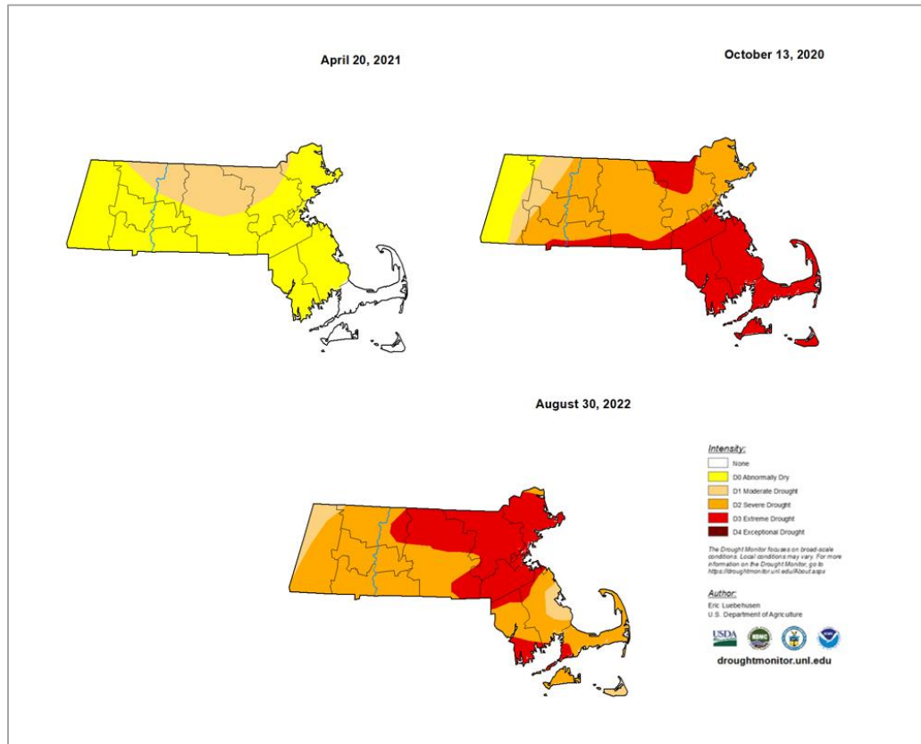
Figure 24. Recent Massachusetts Drought Events (2018-2023)
