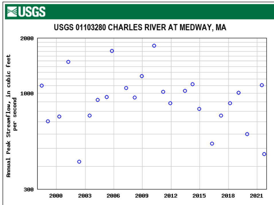
Figure 16. USGS Flood Gage Discharge Data for Charles River at Medway
