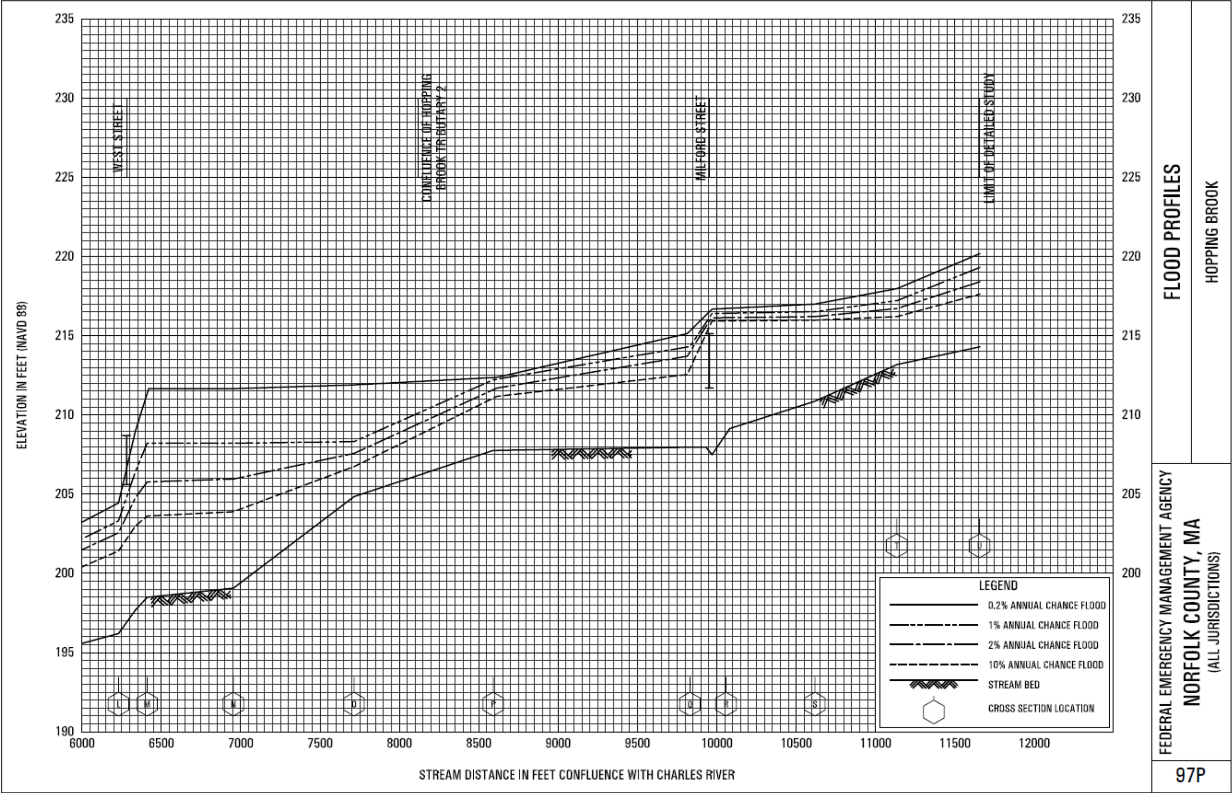
FIS Flood Profile for Hopping Brook in Medway, 97P
