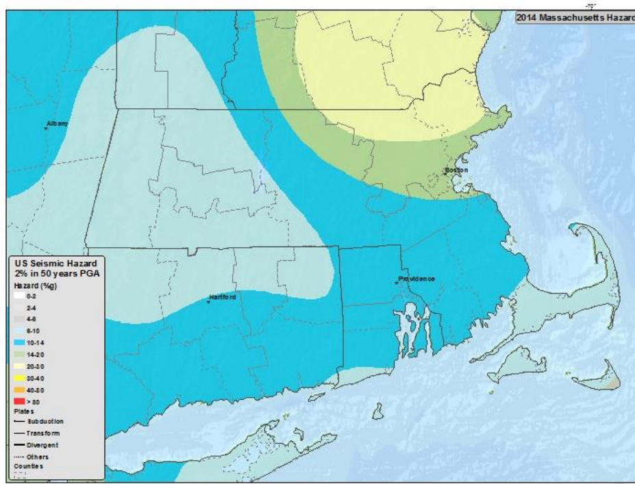
Figure 27. Massachusetts Seismic Hazard Map (2014)
