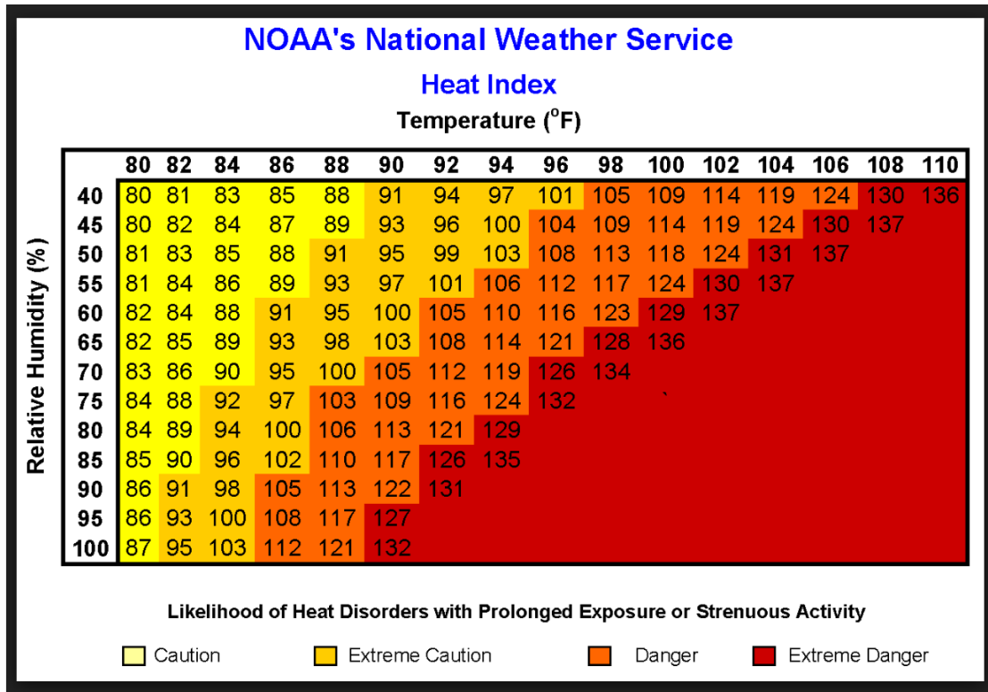
Figure 29. Heat Index Chart
