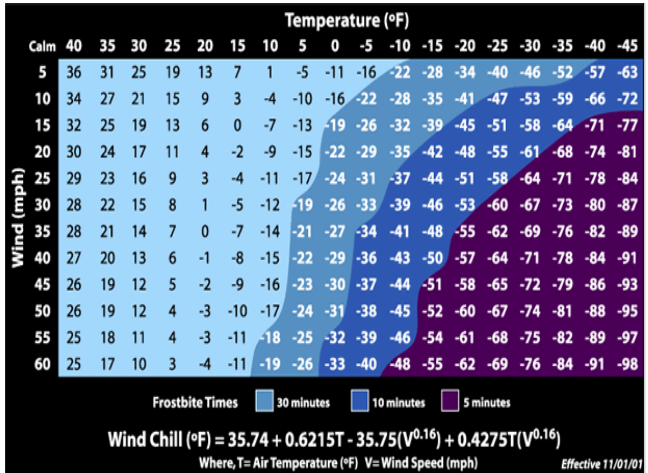
Figure 28. Wind Chill Temperature Index and Frostbite Risk
