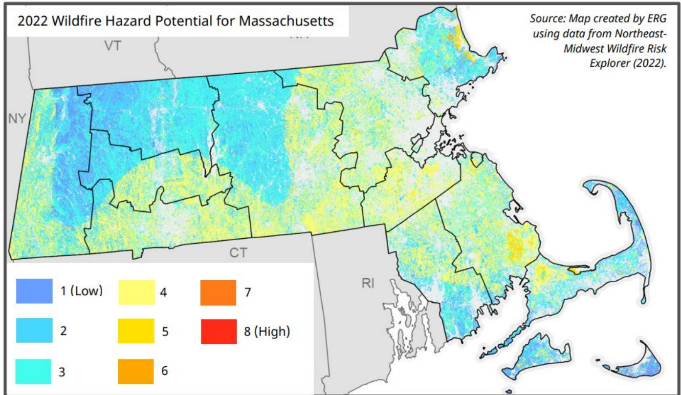
Figure 30. 2022 Wildfire Hazard Potential for Massachusetts
