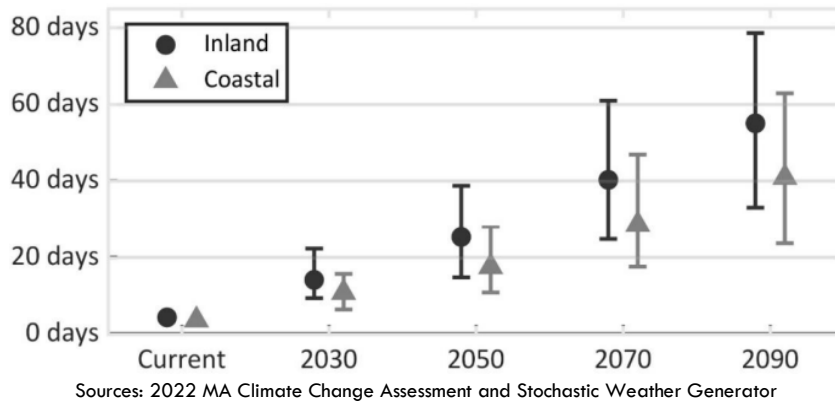
Figure 10. Change in the Annual Number of Days Over 90°F Compared to Today
