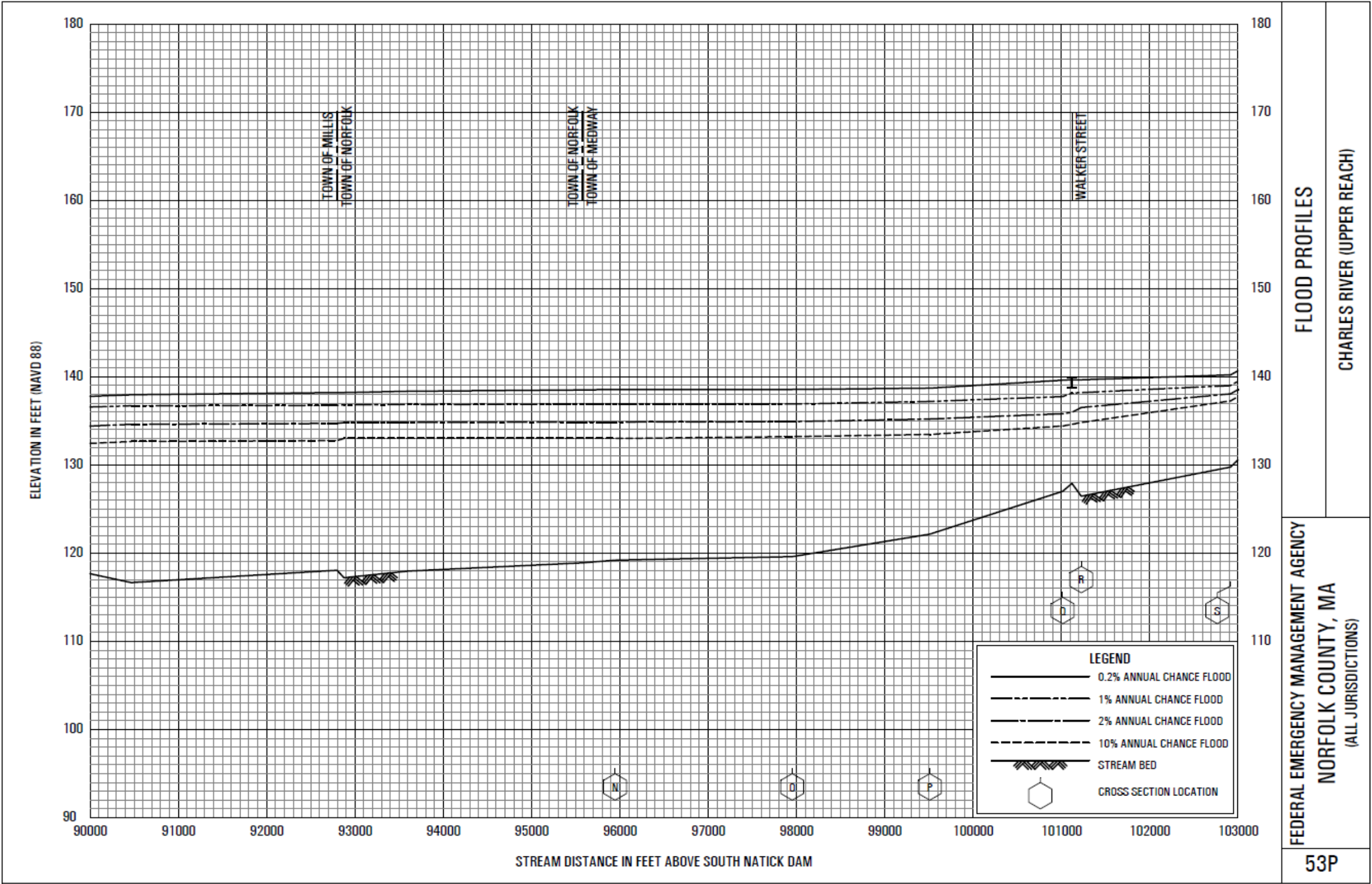
FIS Flood Profile for Charles River Upper Reach in Medway, 53P
