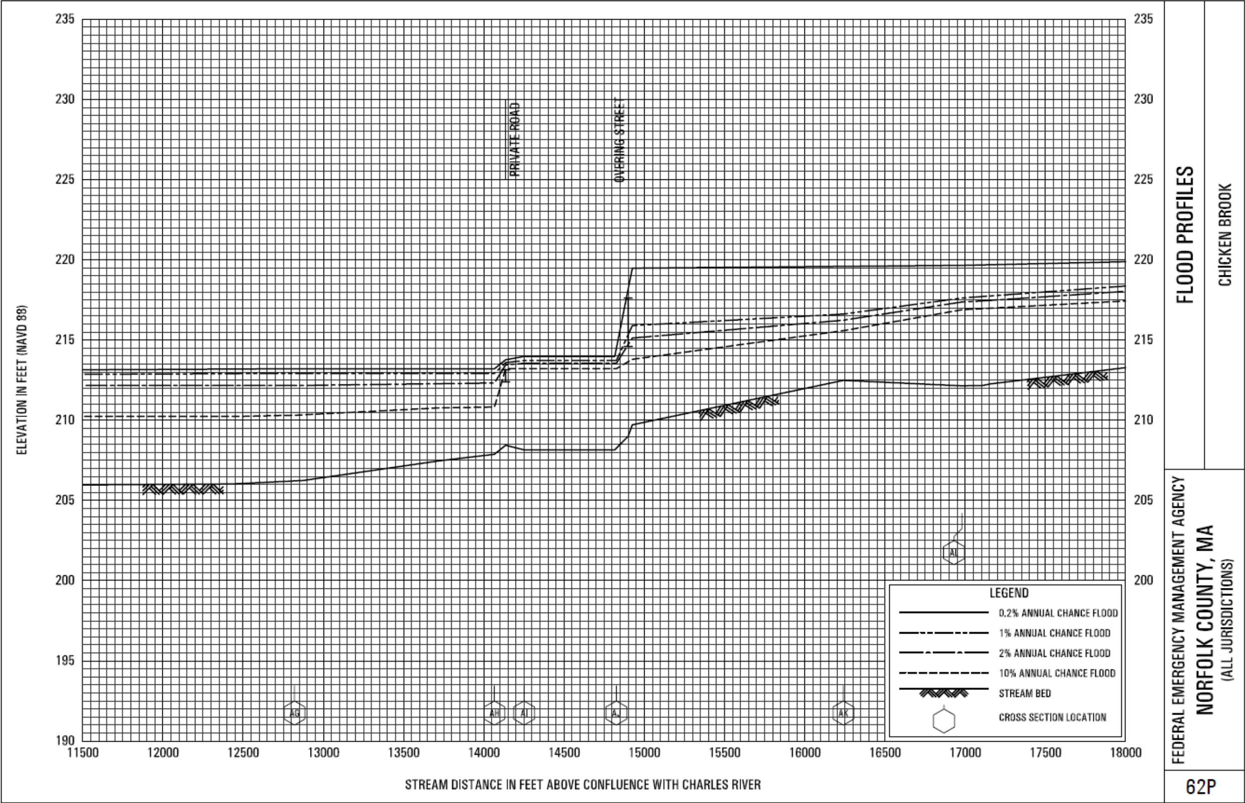
FIS Flood Profile for Chicken Brook in Medway, 62P
