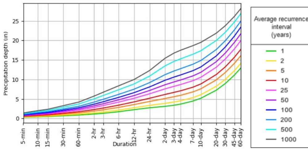
Figure 26. Depth-Duration Frequency Curve
