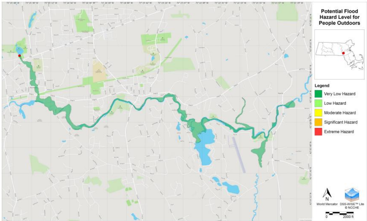
Figure 21. Potential Flood Hazard Level for People Outdoors
