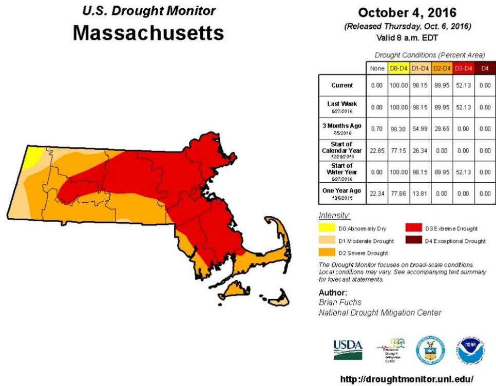
Figure 23. Extreme Drought Conditions in Massachusetts 2016
