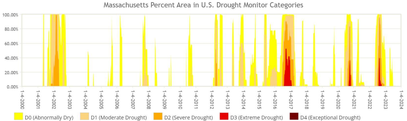
Figure 22. Percent Area in Massachusetts with Drought Conditions 2000-2023
