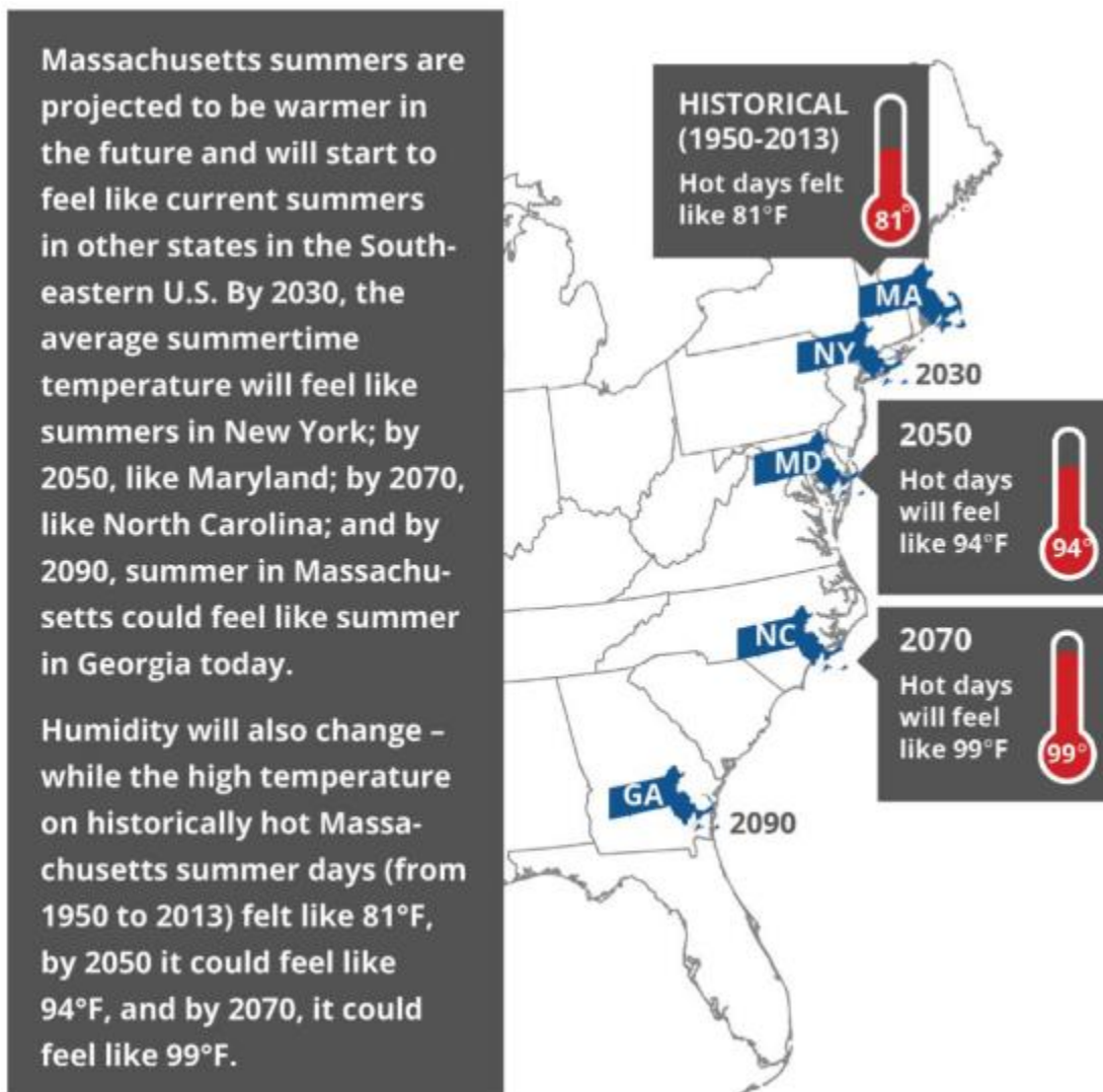
Figure 11. Change in Average Summertime Temperatures for Massachusetts
