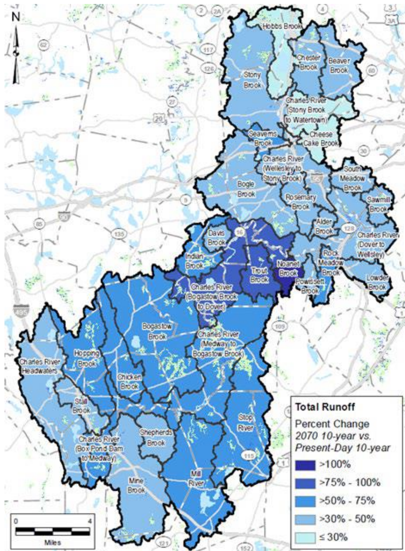
Figure 20. Percent Increase in Total Runoff Volume During the 2070 10-year Event Versus the Baseline 10-year Event, by Sub-Basin
