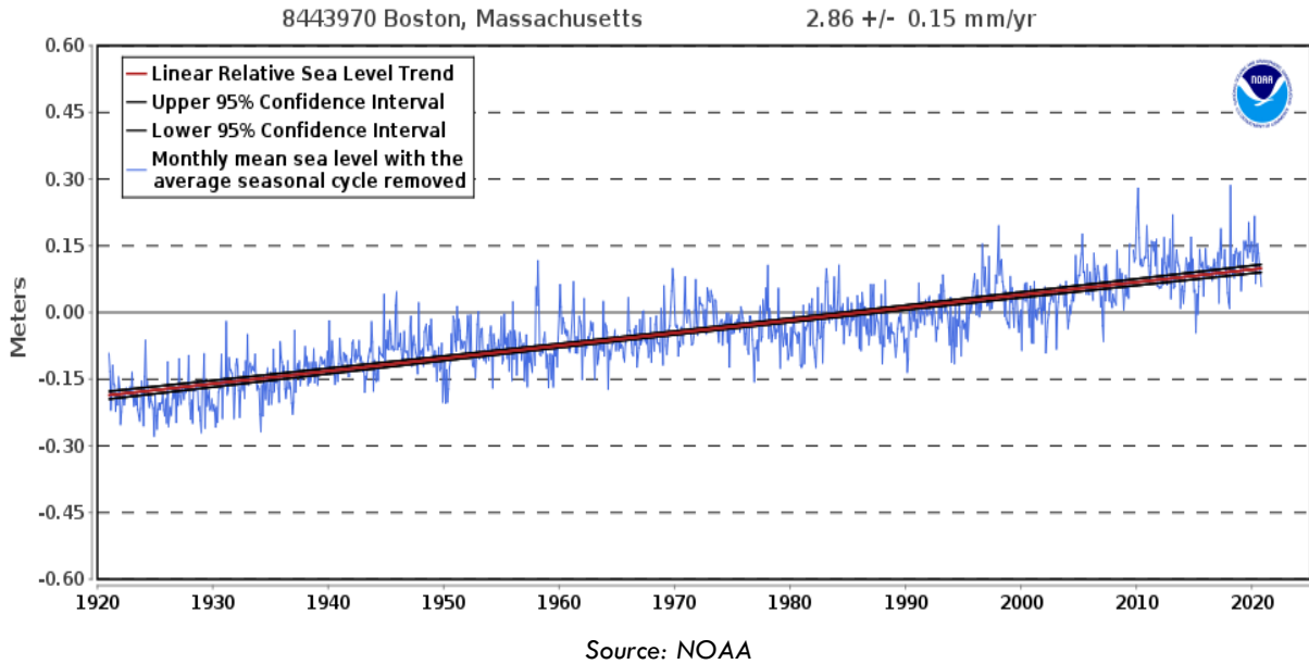
Figure 15. Observed Increase in Sea Level Rise
