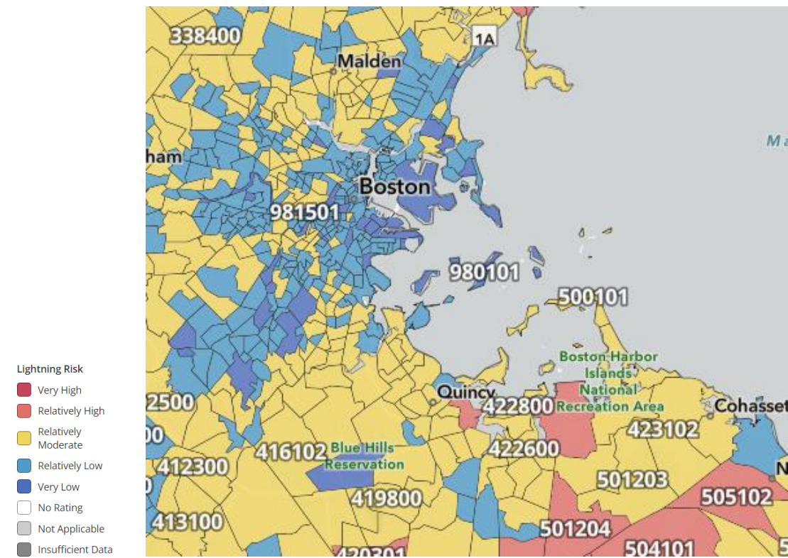
Figure 25. National Risk Index for Lightning
