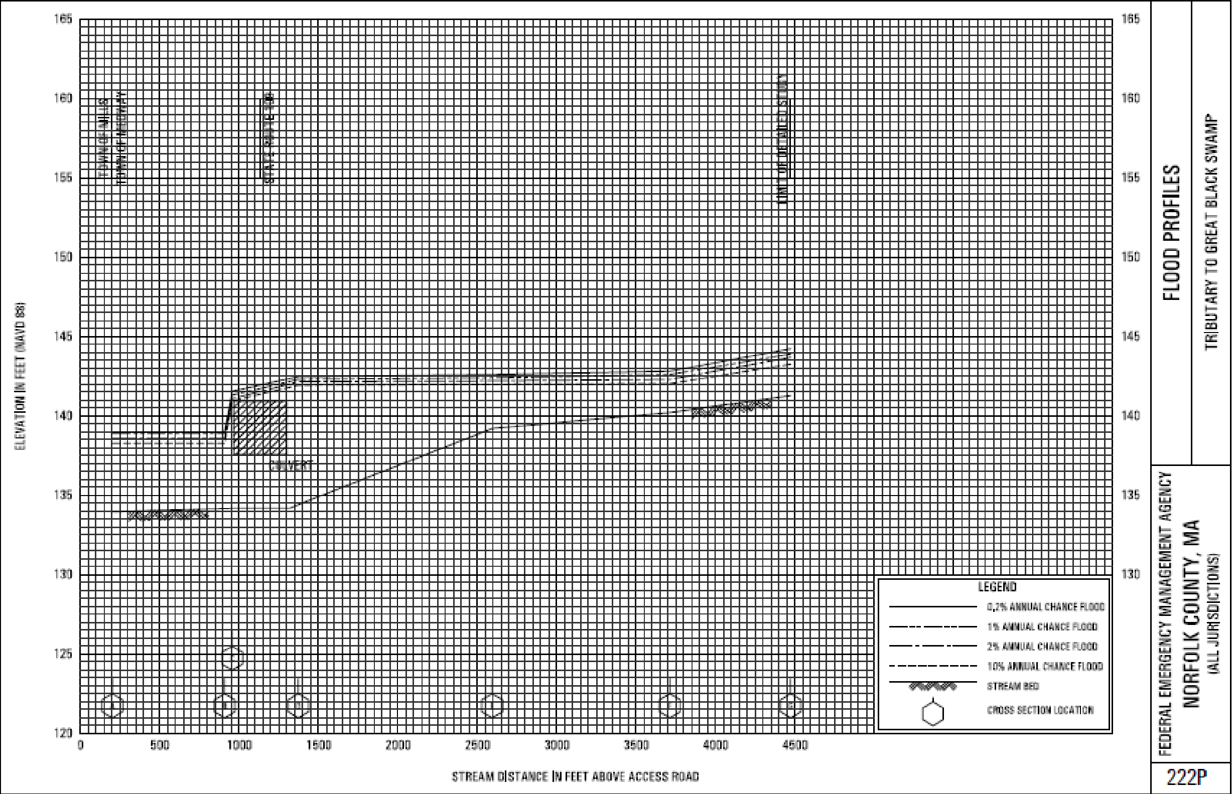
FIS Flood Profile for Tributary of Great Black Swamp in Medway, 222P
