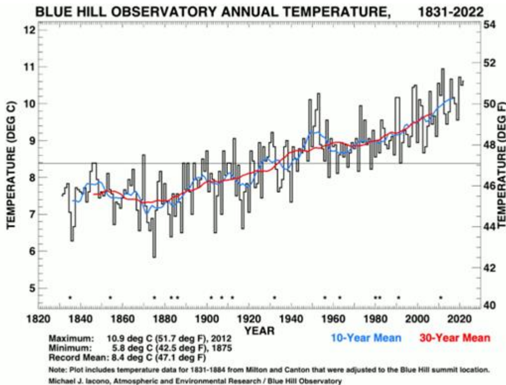
Figure 9. Observed Increase in Temperature
