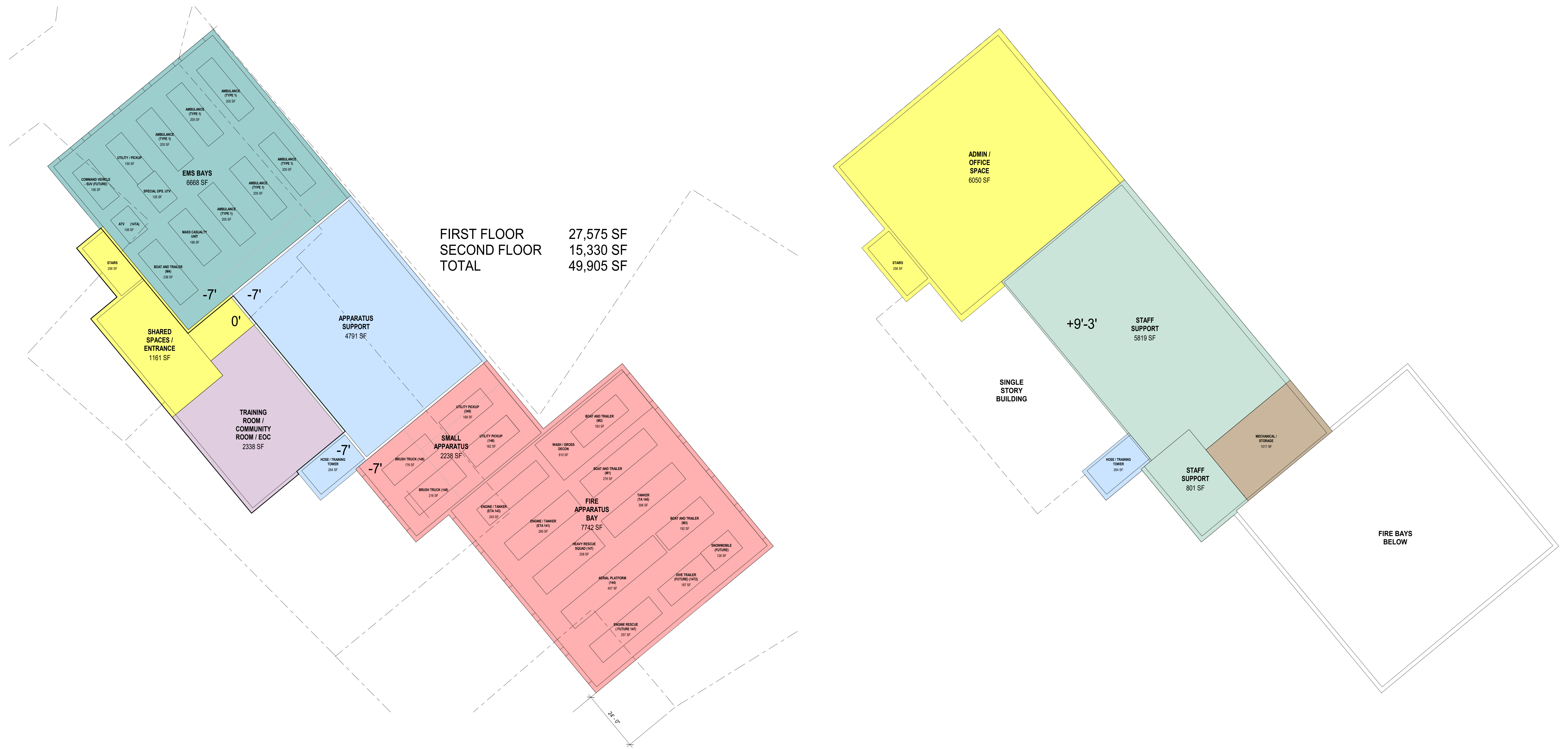
1 EXISTING STATION SITE - FIRST FLOOR CONCEPT 5 SCALE: 1/16" = 1'-0"
