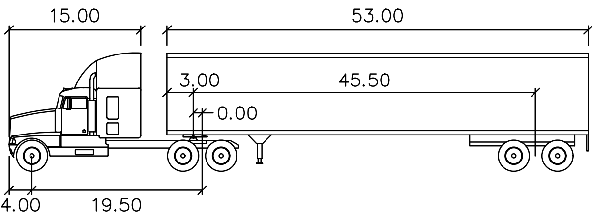
WB-67
