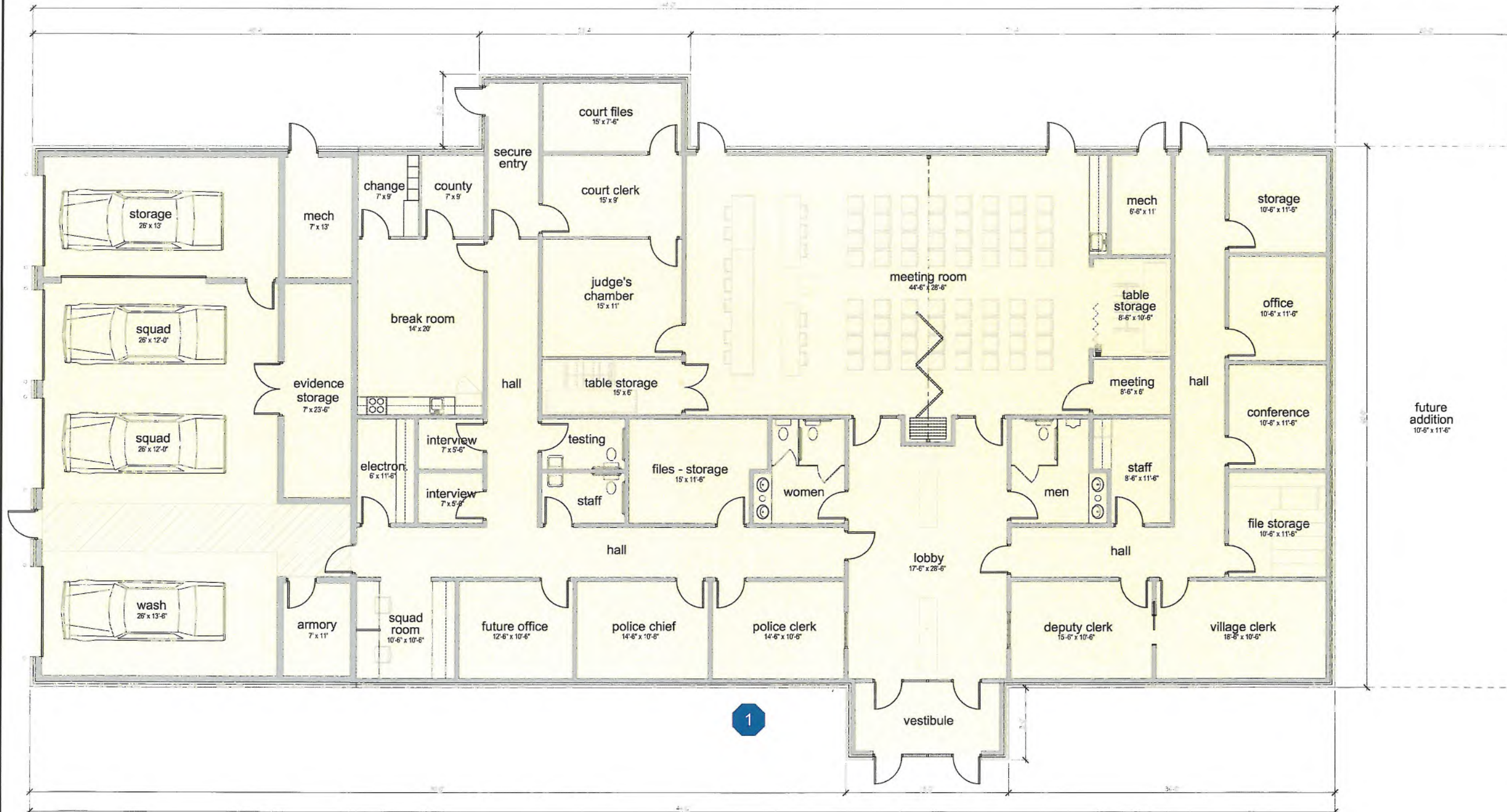
1 new town hall conceptual floor plan 3/16" = 1'-0" NORTH
