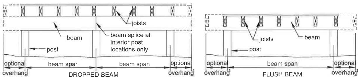
Figure 3 BEAM TYPES
