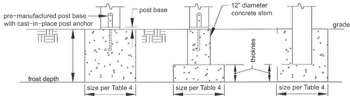
Figure 1 FOOTINGS
