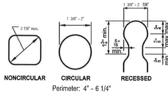
Figure 34 HANDRAIL GRASPABILITY
