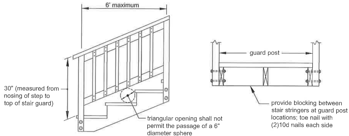
Figure 32 STAIR GUARDS
