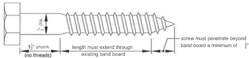
Figure 16 LAG SCREW
