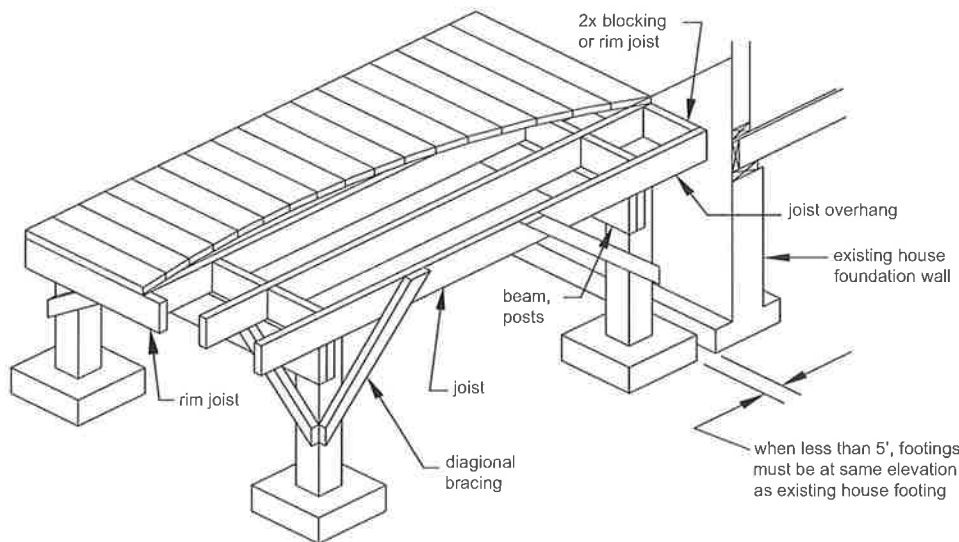
Figure 17 FREE-STANDING DECK
