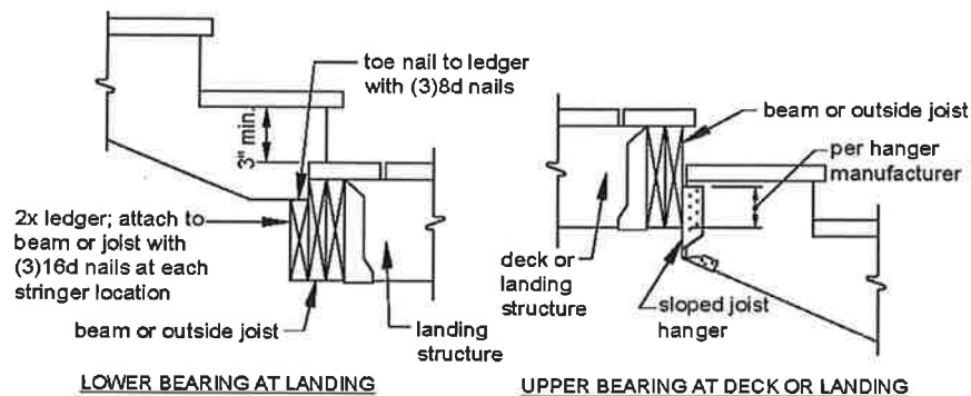
Figure 28 STRINGER BEARING
