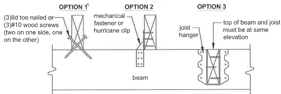
Figure 8 JOIST-TO-BEAM CONNECTIONS
