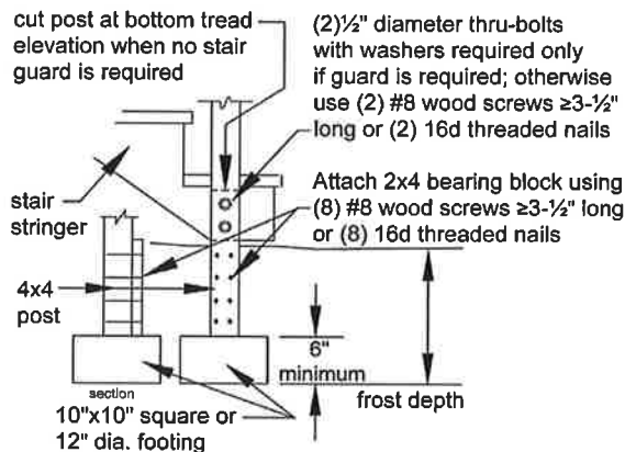
Figure 29 STRINGER BEARING
