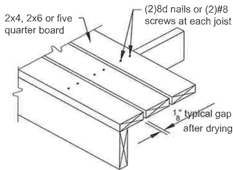
Figure 22 TYPICAL DECKING
