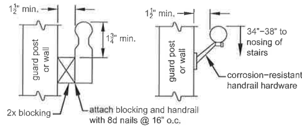
Figure 34 HANDRAIL GRASPABILITY
