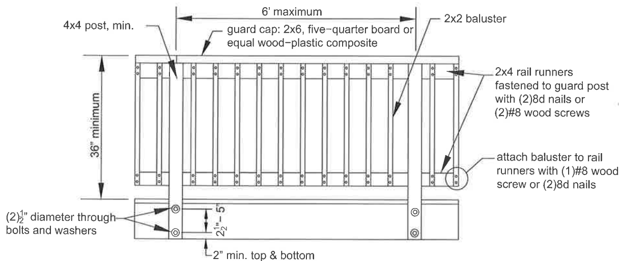
Figure 24 GUARDS
