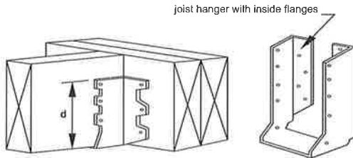
Figure 9 JOIST HANGERS
