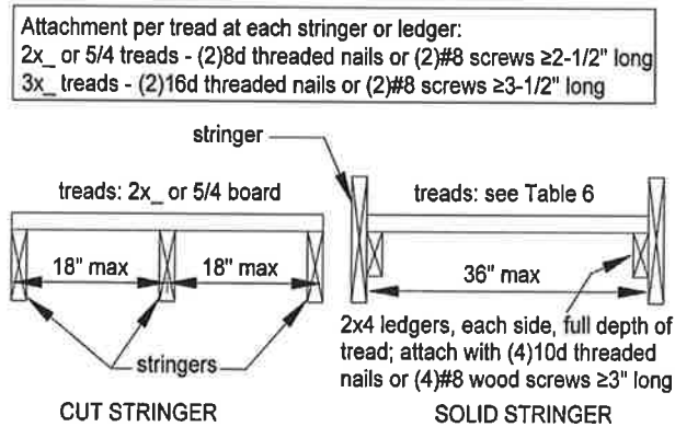
Figure 31 STAIRWAY TREADS
