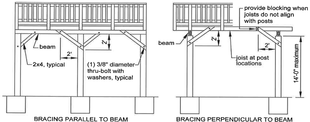
Figure 18 DIAGONAL BRACING REQUIREMENTS
