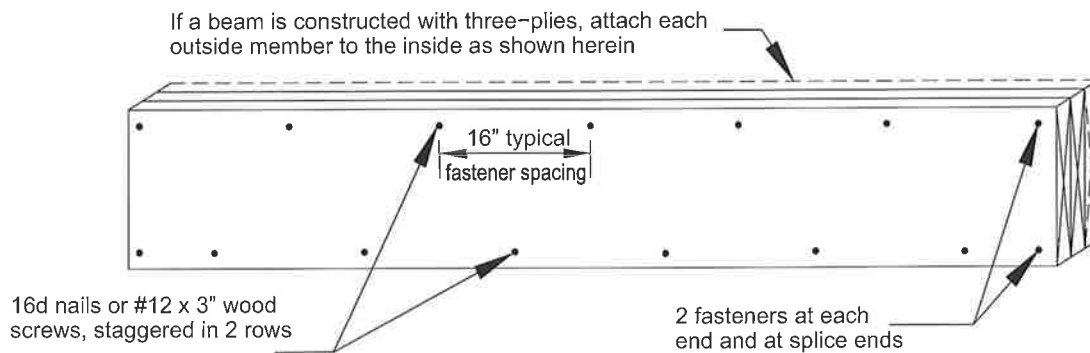
Figure 4 BEAM ASSEMBLY
