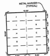
TYPICAL GRAVESITE LAYOUT SCALE: NONE
