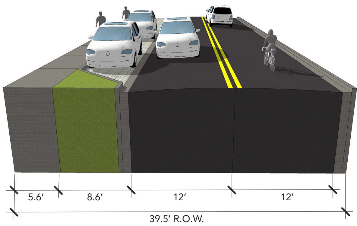
Water Street (39.5' ROW) Section with Parking and Walk on One Side
