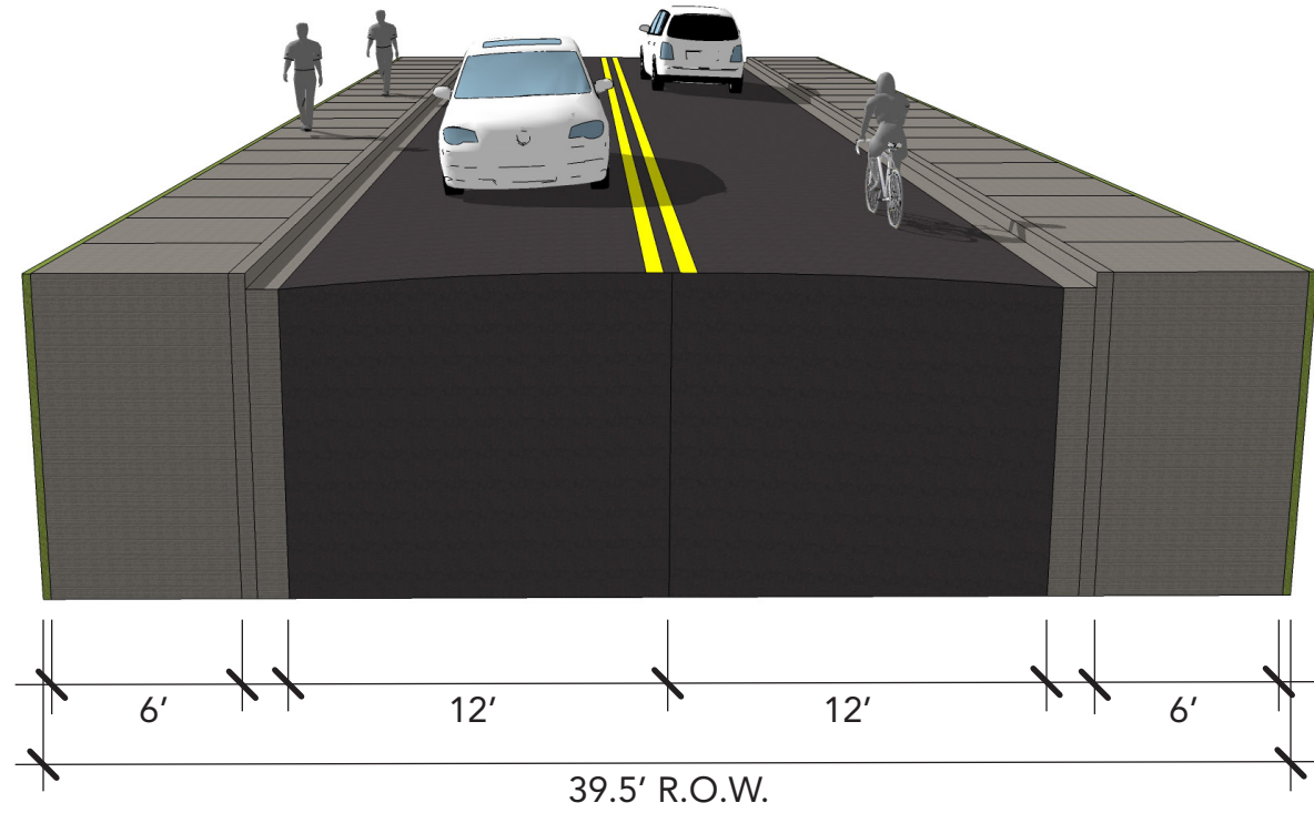
Water Street (39.5' ROW) Section with Walks on Each Side
