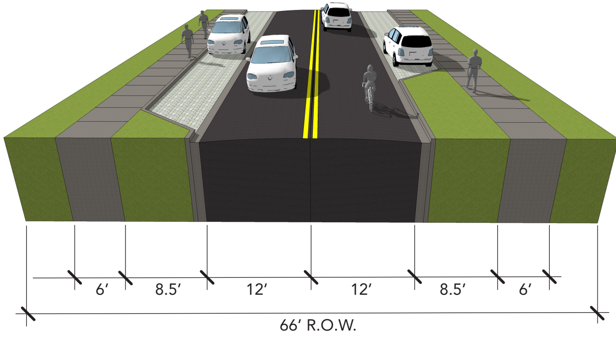
Water Street (66' ROW) Section with Optional Parking & Walks
