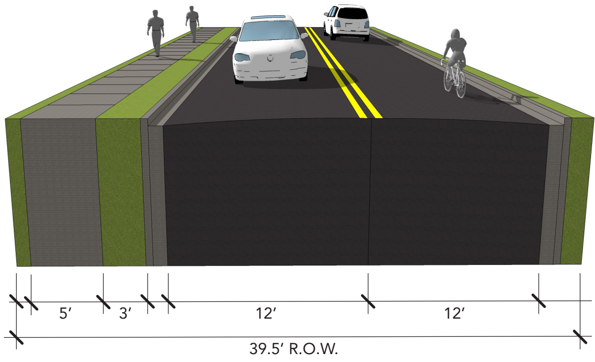
Water Street (39.5' ROW) Section with Walk on One Side
