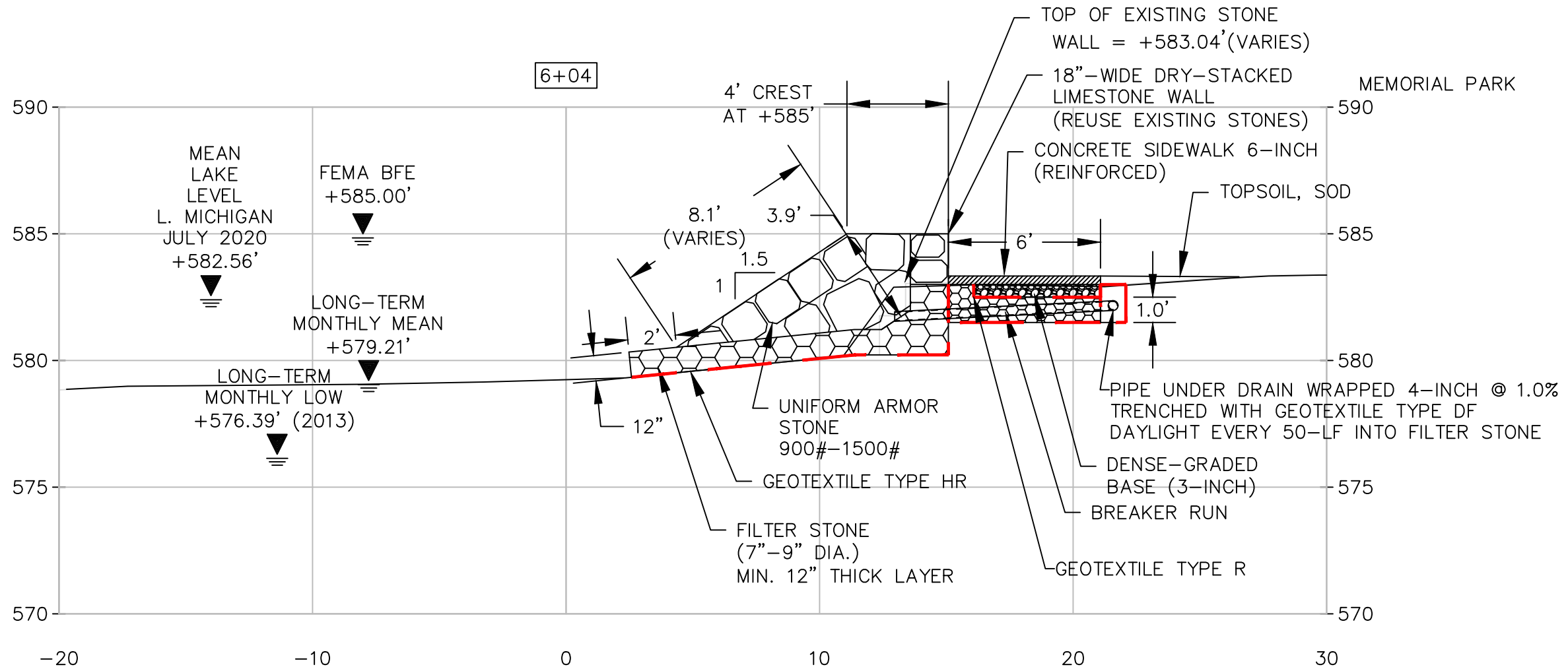
CROSS SECTION 6+04 TYPICAL FOR CENTRAL SITE
