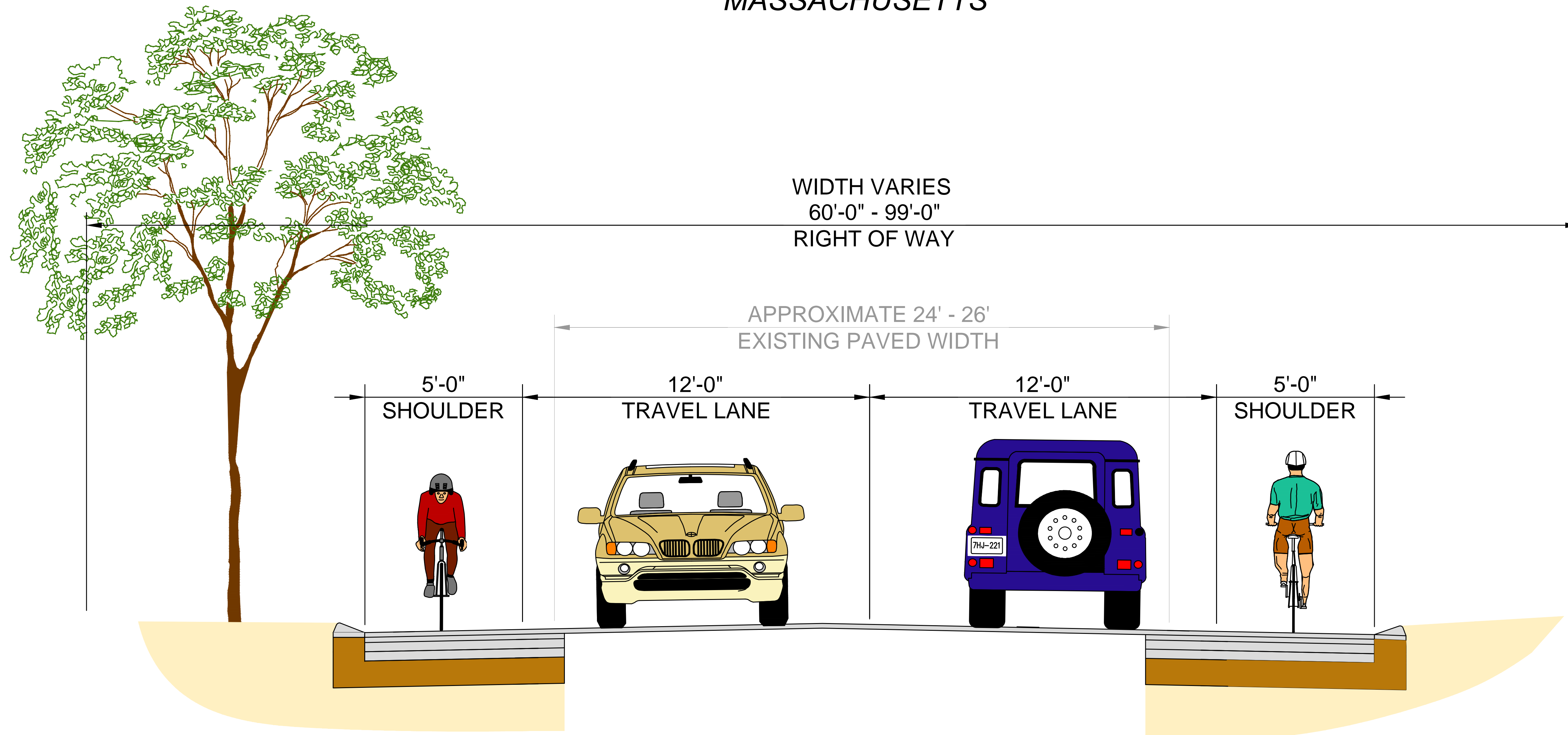
TYPICAL SECTION WEST MAIN STREET (ROUTE 9)
