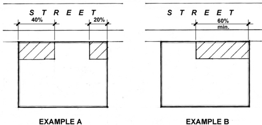
FIGURE 8-4C-4 TWO DIFFERENT WAYS TO ACHIEVE STREET FRONTAGE EXAMPLES
