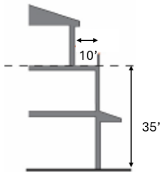
FIGURE 8-2B-1 ILLUSTRATION OF STEP BACK
