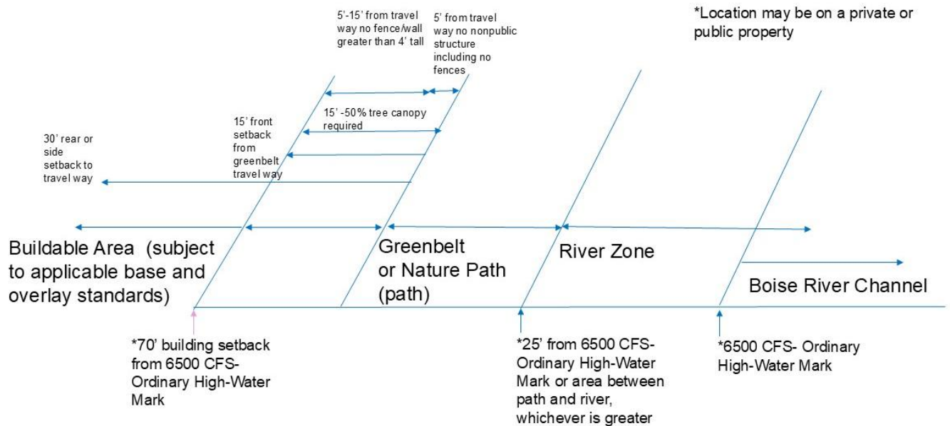
FIGURE 8-4M-2 AREAS WITH GREENBELT OR NATURE PATH
