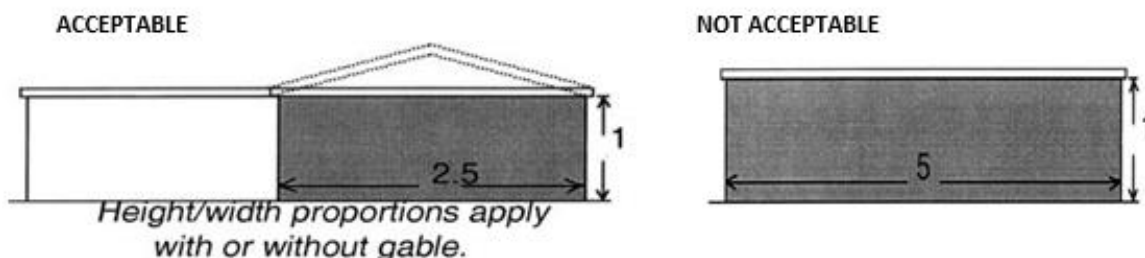
Figure 8-4C-5 Acceptable A and Not Acceptable Wall Plane Dimensions Examples
