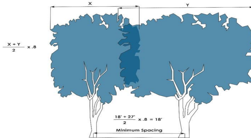
FIGURE 8-4I-1 ILLUSTRATION OF TREE SPACING
