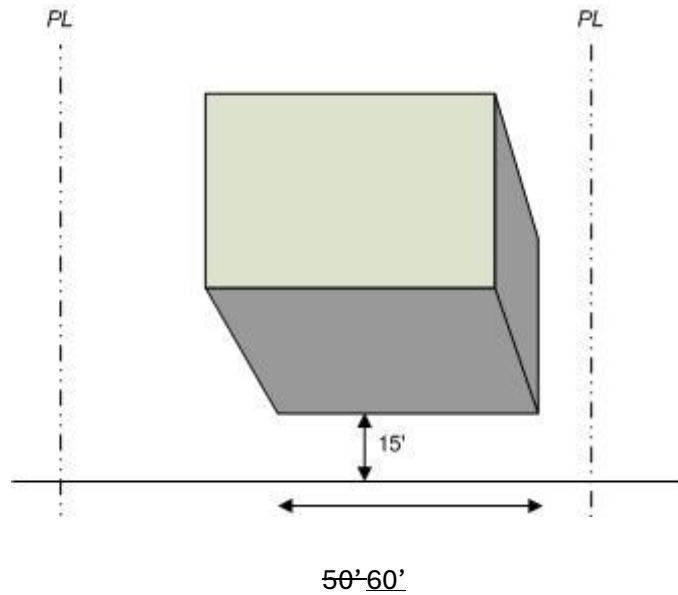
FIGURE 8-4C-2: ILLUSTRATION OF MAXIMUM SETBACK ALONG STREET FRONT
