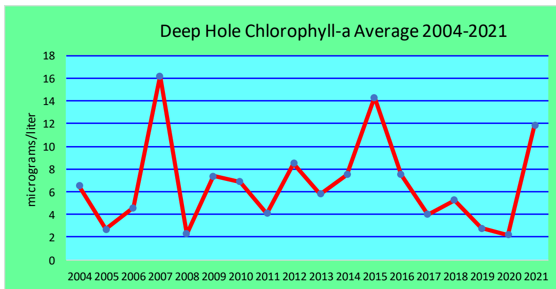
Figure 5: Average Chlorophyll-a Levels in Peppermill Lake 2004-2021
