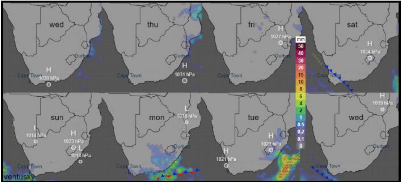
Available at: file:///C:/Users/User/Downloads/rmddailyweather%20(21).pdf
