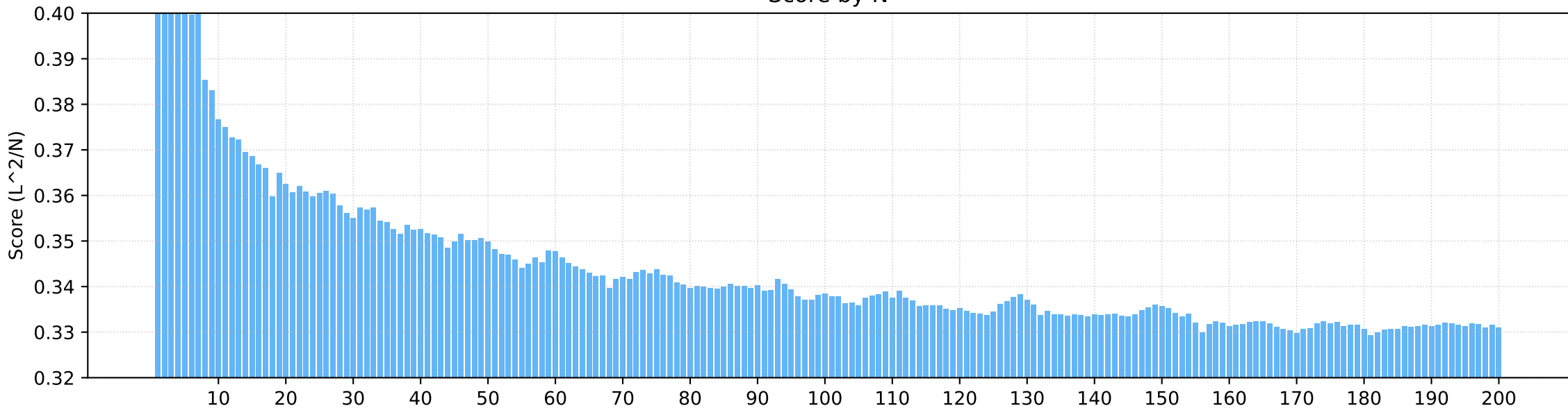
Packing density by N
