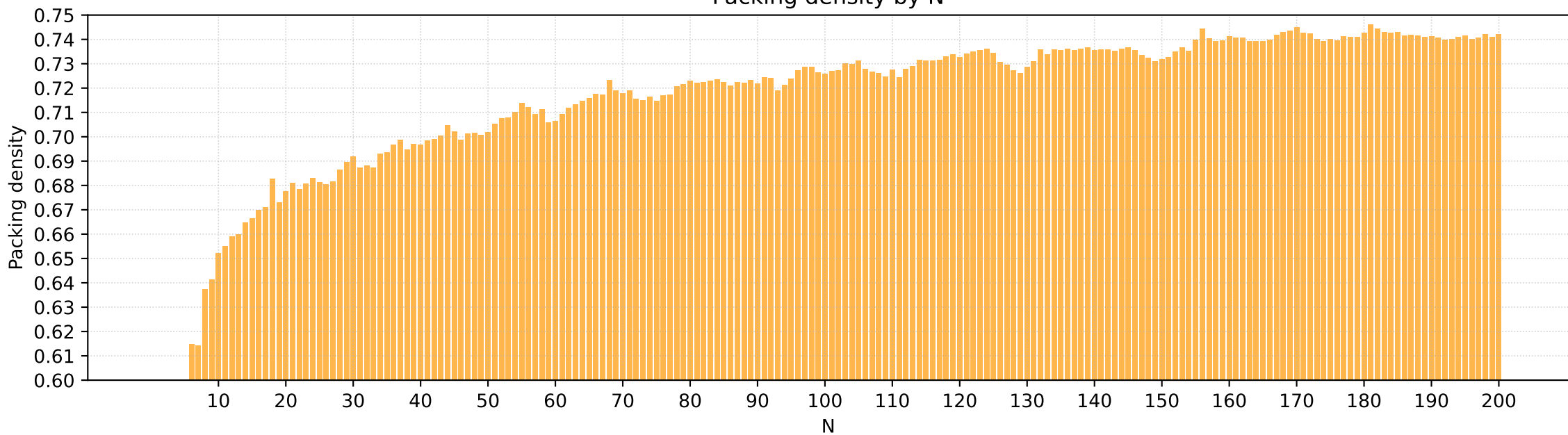
Packing density by N
